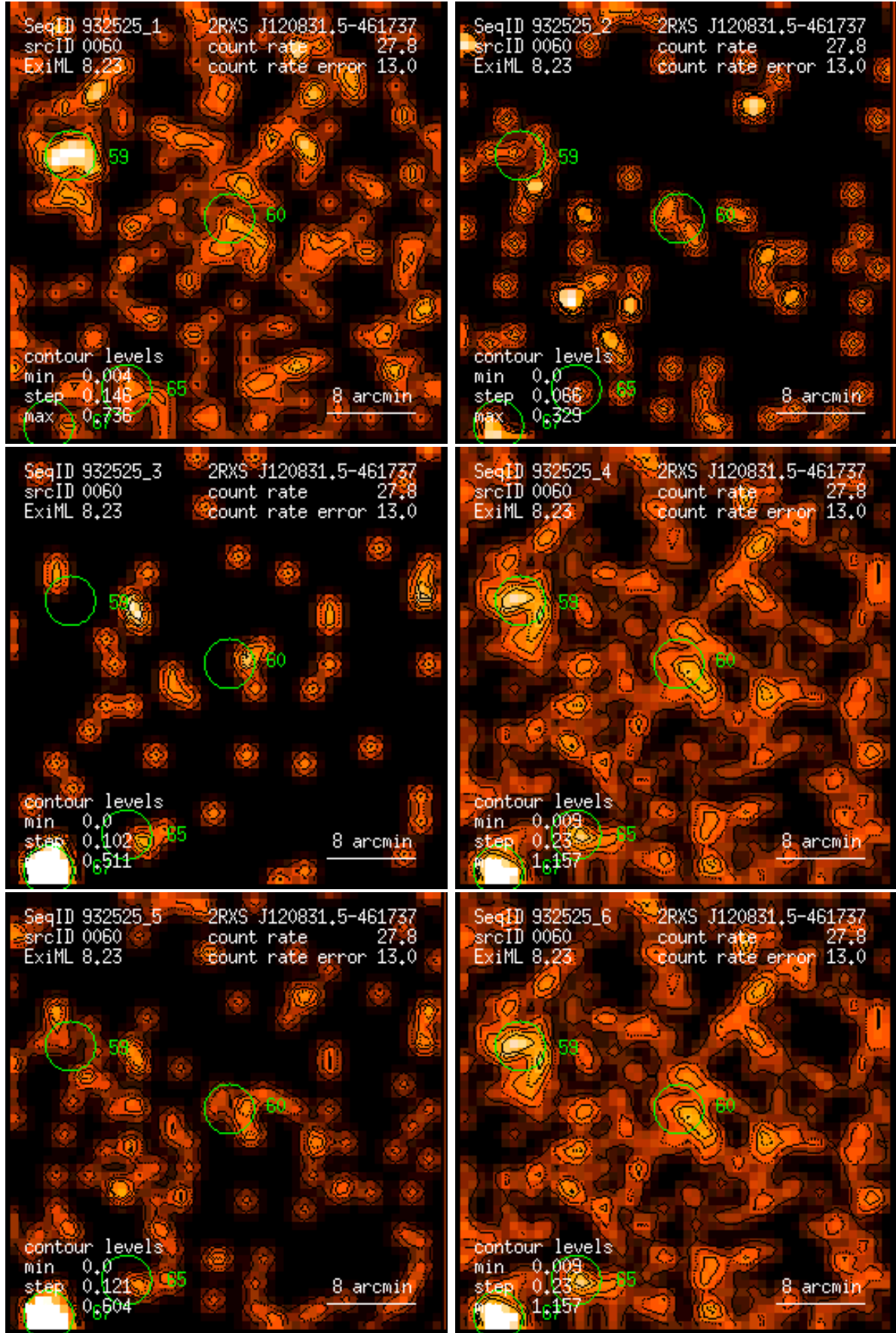
Figure 60: RASS 932525: detection 0060: band rate images, Gaussian filter: (1) PSPC channels 11 – 41, (2) 52 – 90, (3) 91 – 201, (4) 11 – 235, (5) 52 – 201, (6) 11 – 201. Broad band rates in counts/ks. Band rate contour levels in counts/ks/arcmin 2 .
