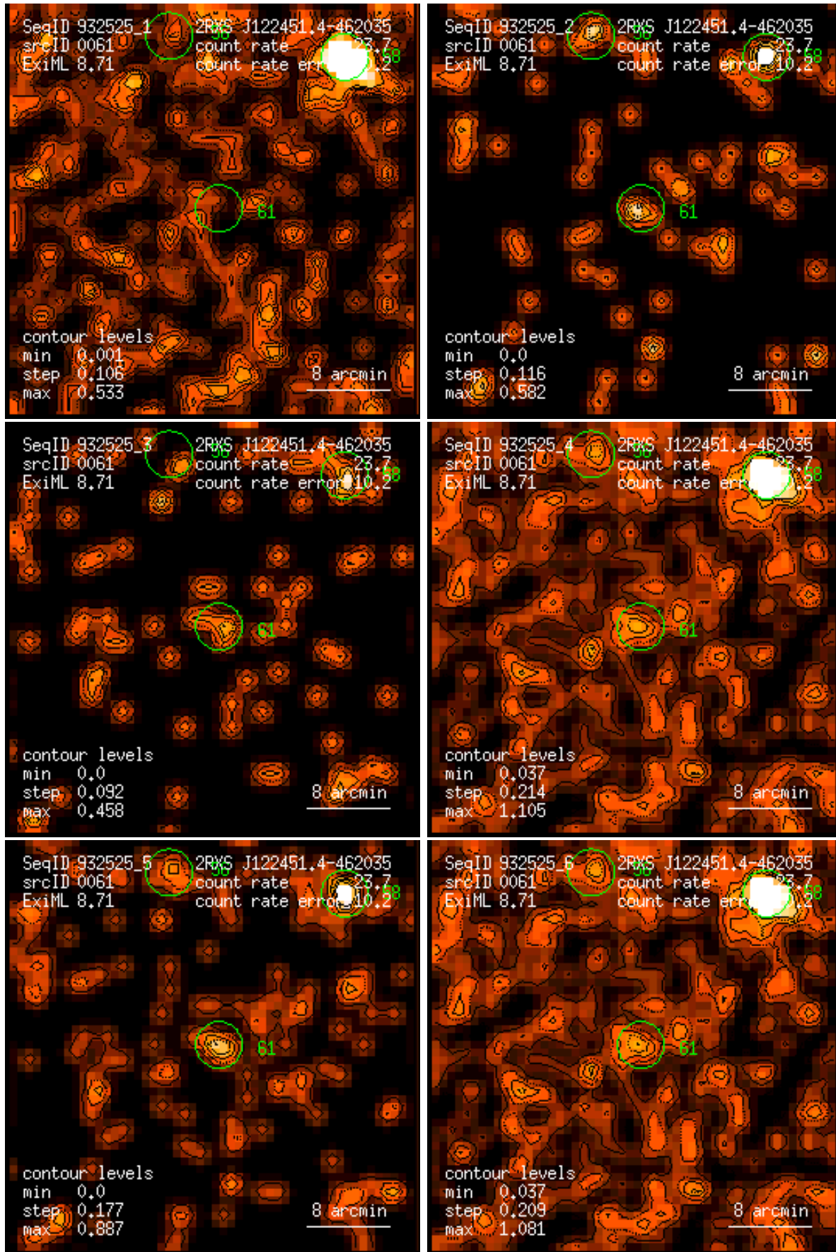
Figure 61: RASS 932525: detection 0061: band rate images, Gaussian filter: (1) PSPC channels 11 – 41, (2) 52 – 90, (3) 91 – 201, (4) 11 – 235, (5) 52 – 201, (6) 11 – 201. Broad band rates in counts/ks. Band rate contour levels in counts/ks/arcmin 2 .
