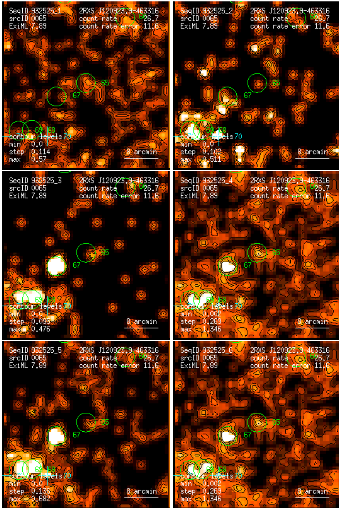
Figure 65: RASS 932525: detection 0065: band rate images, Gaussian filter: (1) PSPC channels 11 – 41, (2) 52 – 90, (3) 91 – 201, (4) 11 – 235, (5) 52 – 201, (6) 11 – 201. Broad band rates in counts/ks. Band rate contour levels in counts/ks/arcmin 2 .
