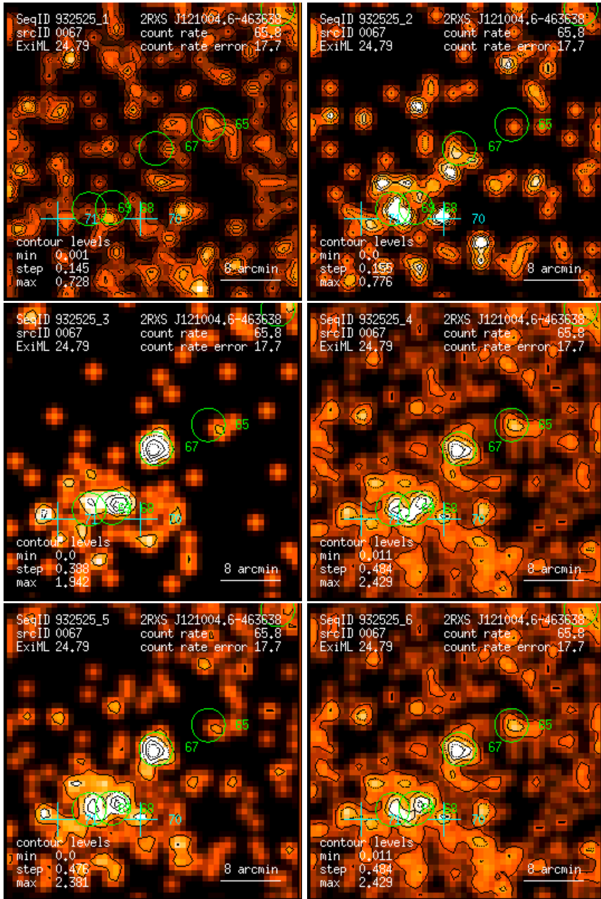
Figure 67: RASS 932525: detection 0067: band rate images, Gaussian filter: (1) PSPC channels 11 – 41, (2) 52 – 90, (3) 91 – 201, (4) 11 – 235, (5) 52 – 201, (6) 11 – 201. Broad band rates in counts/ks. Band rate contour levels in counts/ks/arcmin 2 .
