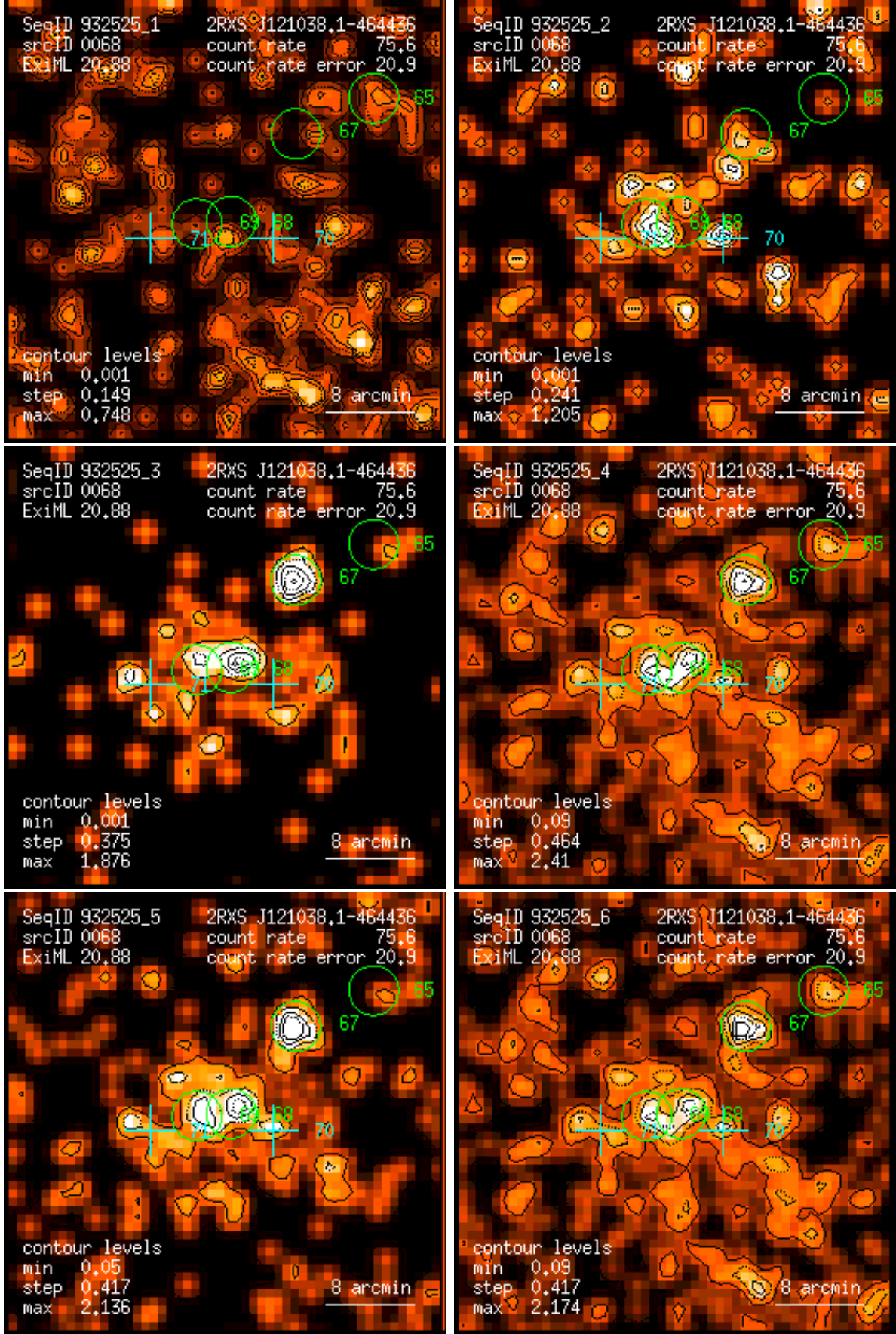
Figure 68: RASS 932525: detection 0068: band rate images, Gaussian filter: (1) PSPC channels 11 – 41, (2) 52 – 90, (3) 91 – 201, (4) 11 – 235, (5) 52 – 201, (6) 11 – 201. Broad band rates in counts/ks. Band rate contour levels in counts/ks/arcmin 2 .
