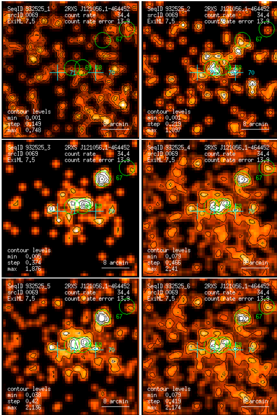
Figure 69: RASS 932525: detection 0069: band rate images, Gaussian filter: (1) PSPC channels 11 – 41, (2) 52 – 90, (3) 91 – 201, (4) 11 – 235, (5) 52 – 201, (6) 11 – 201. Broad band rates in counts/ks. Band rate contour levels in counts/ks/arcmin 2 .
