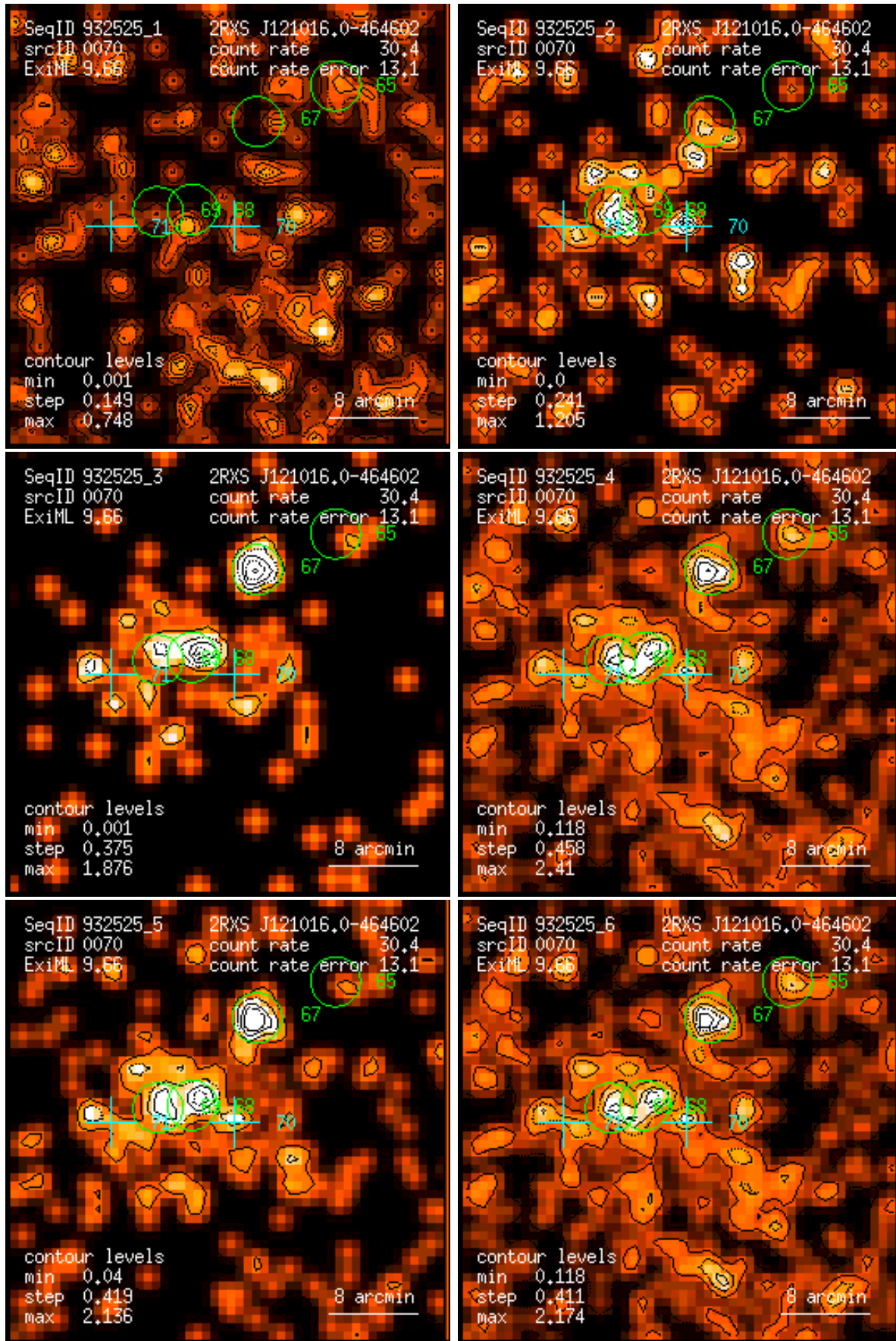
Figure 70: RASS 932525: detection 0070: band rate images, Gaussian filter: (1) PSPC channels 11 – 41, (2) 52 – 90, (3) 91 – 201, (4) 11 – 235, (5) 52 – 201, (6) 11 – 201. Broad band rates in counts/ks. Band rate contour levels in counts/ks/arcmin 2 .
