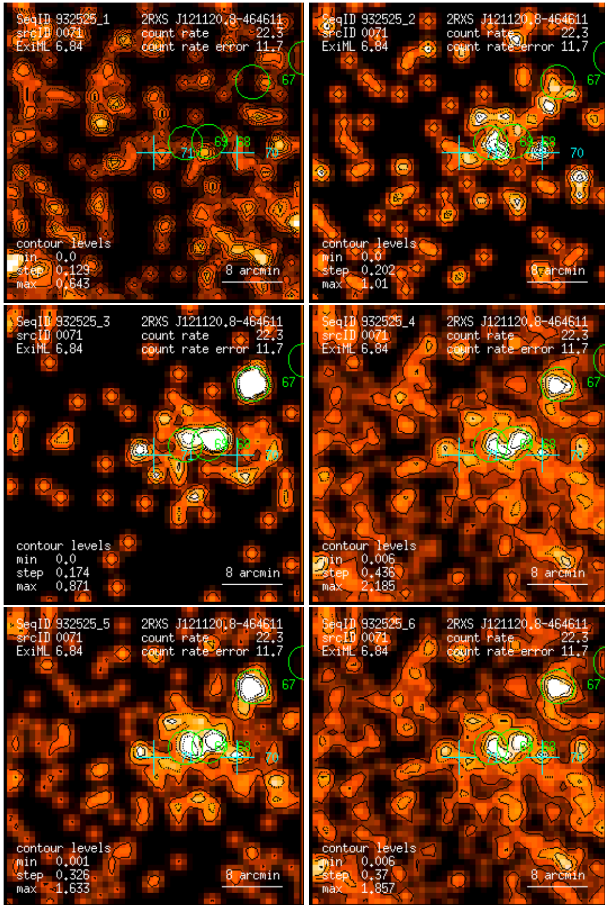
Figure 71: RASS 932525: detection 0071: band rate images, Gaussian filter: (1) PSPC channels 11 – 41, (2) 52 – 90, (3) 91 – 201, (4) 11 – 235, (5) 52 – 201, (6) 11 – 201. Broad band rates in counts/ks. Band rate contour levels in counts/ks/arcmin 2 .
