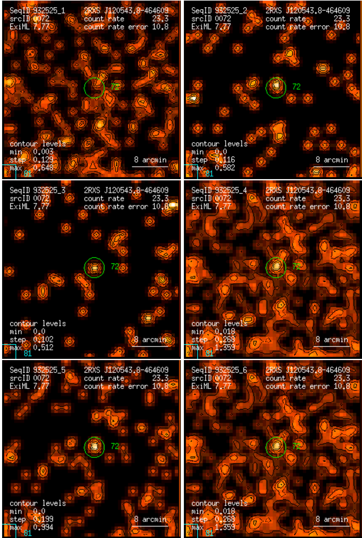
Figure 72: RASS 932525: detection 0072: band rate images, Gaussian filter: (1) PSPC channels 11 – 41, (2) 52 – 90, (3) 91 – 201, (4) 11 – 235, (5) 52 – 201, (6) 11 – 201. Broad band rates in counts/ks. Band rate contour levels in counts/ks/arcmin 2 .
