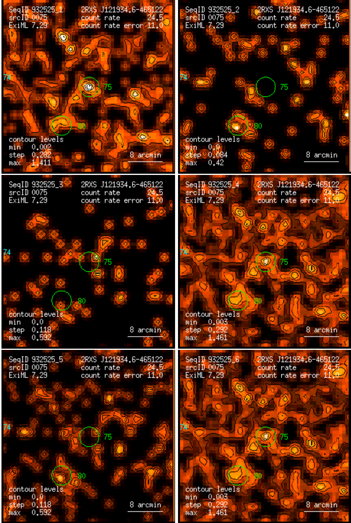
Figure 75: RASS 932525: detection 0075: band rate images, Gaussian filter: (1) PSPC channels 11 – 41, (2) 52 – 90, (3) 91 – 201, (4) 11 – 235, (5) 52 – 201, (6) 11 – 201. Broad band rates in counts/ks. Band rate contour levels in counts/ks/arcmin 2 .
