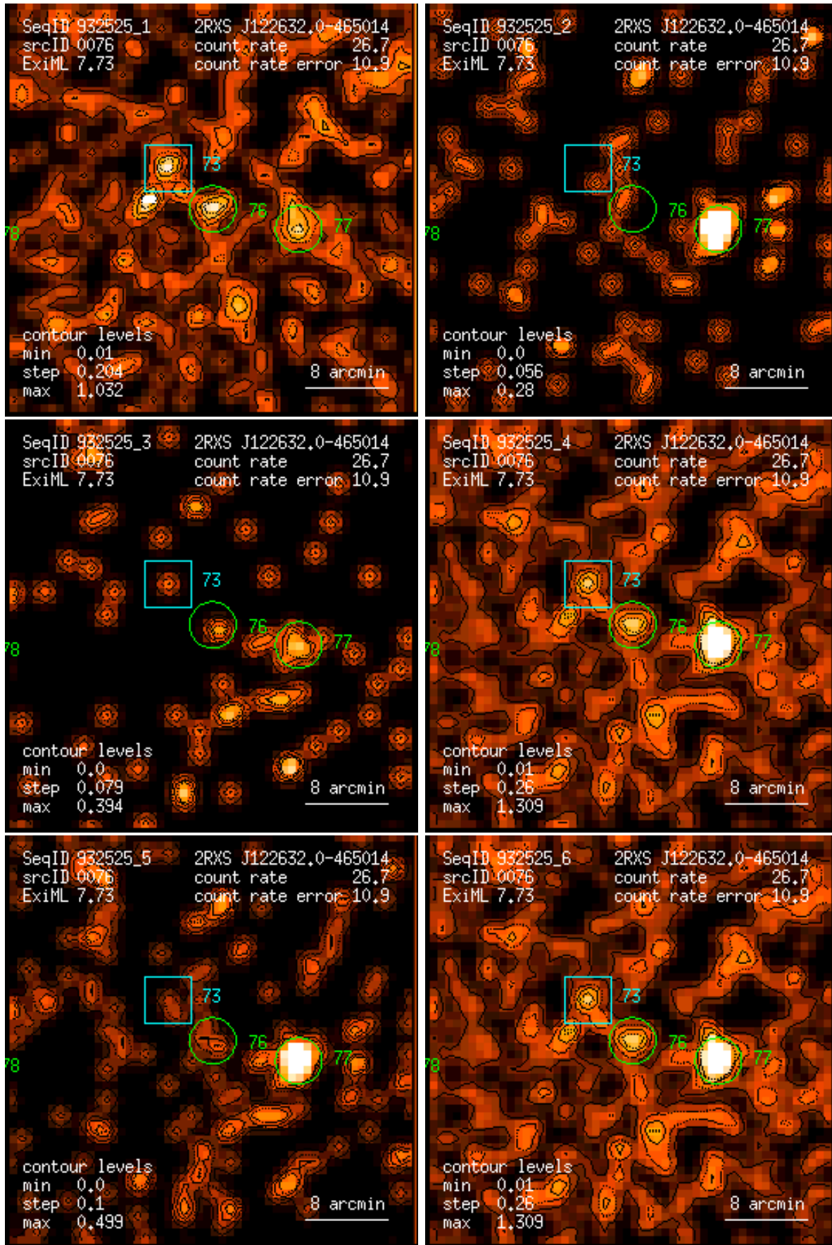
Figure 76: RASS 932525: detection 0076: band rate images, Gaussian filter: (1) PSPC channels 11 – 41, (2) 52 – 90, (3) 91 – 201, (4) 11 – 235, (5) 52 – 201, (6) 11 – 201. Broad band rates in counts/ks. Band rate contour levels in counts/ks/arcmin 2 .
