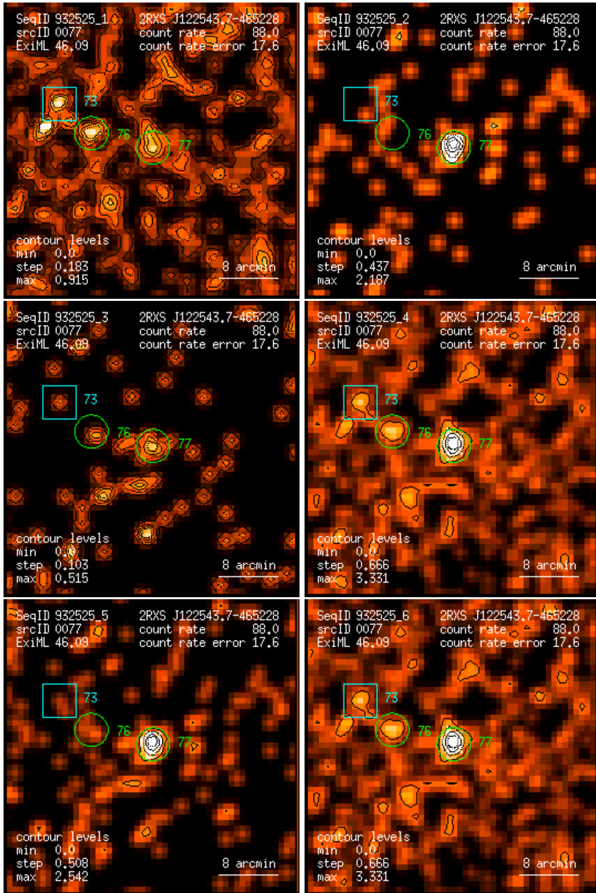
Figure 77: RASS 932525: detection 0077: band rate images, Gaussian filter: (1) PSPC channels 11 – 41, (2) 52 – 90, (3) 91 – 201, (4) 11 – 235, (5) 52 – 201, (6) 11 – 201. Broad band rates in counts/ks. Band rate contour levels in counts/ks/arcmin 2 .
