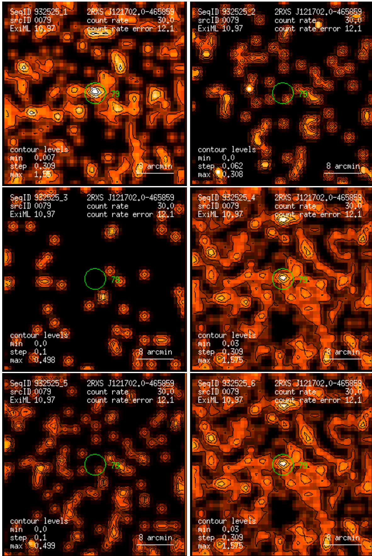
Figure 79: RASS 932525: detection 0079: band rate images, Gaussian filter: (1) PSPC channels 11 – 41, (2) 52 – 90, (3) 91 – 201, (4) 11 – 235, (5) 52 – 201, (6) 11 – 201. Broad band rates in counts/ks. Band rate contour levels in counts/ks/arcmin 2 .
