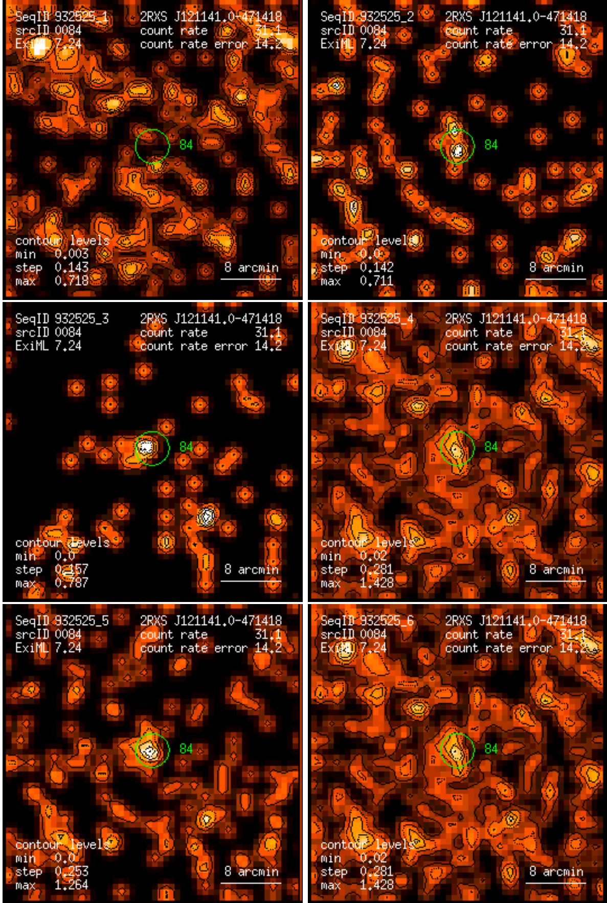
Figure 84: RASS 932525: detection 0084: band rate images, Gaussian filter: (1) PSPC channels 11 – 41, (2) 52 – 90, (3) 91 – 201, (4) 11 – 235, (5) 52 – 201, (6) 11 – 201. Broad band rates in counts/ks. Band rate contour levels in counts/ks/arcmin 2 .
