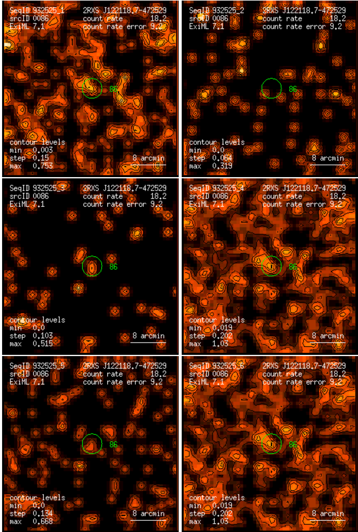
Figure 86: RASS 932525: detection 0086: band rate images, Gaussian filter: (1) PSPC channels 11 – 41, (2) 52 – 90, (3) 91 – 201, (4) 11 – 235, (5) 52 – 201, (6) 11 – 201. Broad band rates in counts/ks. Band rate contour levels in counts/ks/arcmin 2 .
