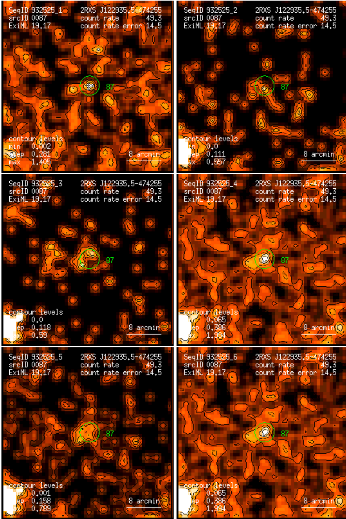
Figure 87: RASS 932525: detection 0087: band rate images, Gaussian filter: (1) PSPC channels 11 – 41, (2) 52 – 90, (3) 91 – 201, (4) 11 – 235, (5) 52 – 201, (6) 11 – 201. Broad band rates in counts/ks. Band rate contour levels in counts/ks/arcmin 2 .
