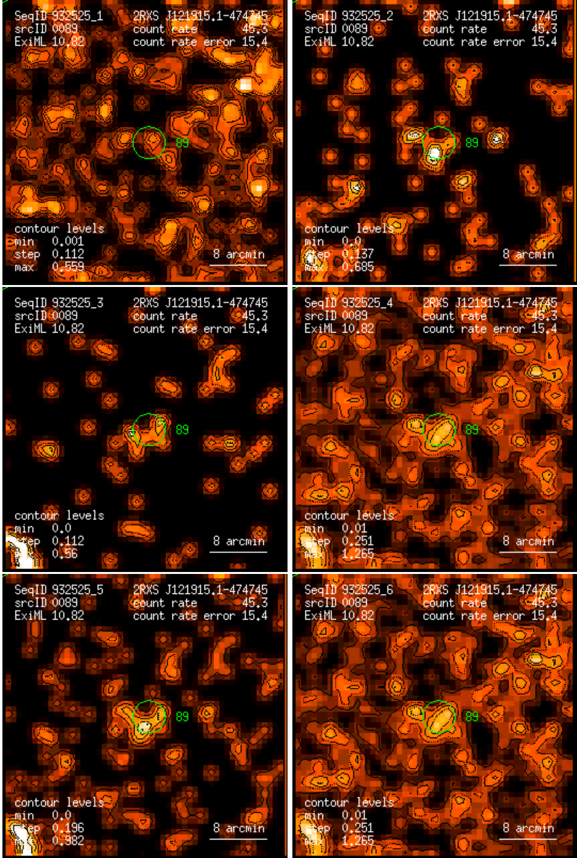
Figure 89: RASS 932525: detection 0089: band rate images, Gaussian filter: (1) PSPC channels 11 – 41, (2) 52 – 90, (3) 91 – 201, (4) 11 – 235, (5) 52 – 201, (6) 11 – 201. Broad band rates in counts/ks. Band rate contour levels in counts/ks/arcmin 2 .
