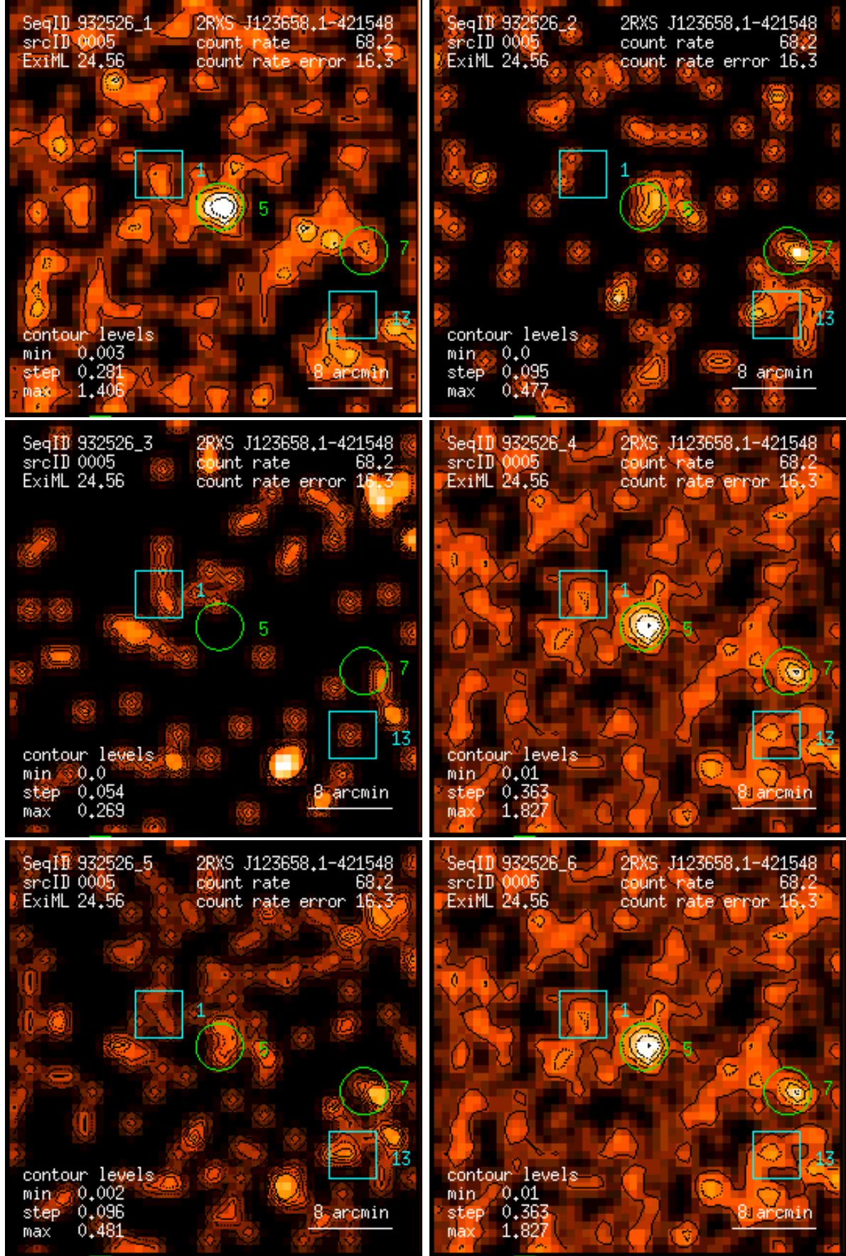
Figure 5: RASS 932526: detection 0005: band rate images, Gaussian filter: (1) PSPC channels 11 – 41, (2) 52 – 90, (3) 91 – 201, (4) 11 – 235, (5) 52 – 201, (6) 11 – 201. Broad band rates in counts/ks. Band rate contour levels in counts/ks/arcmin 2 .
