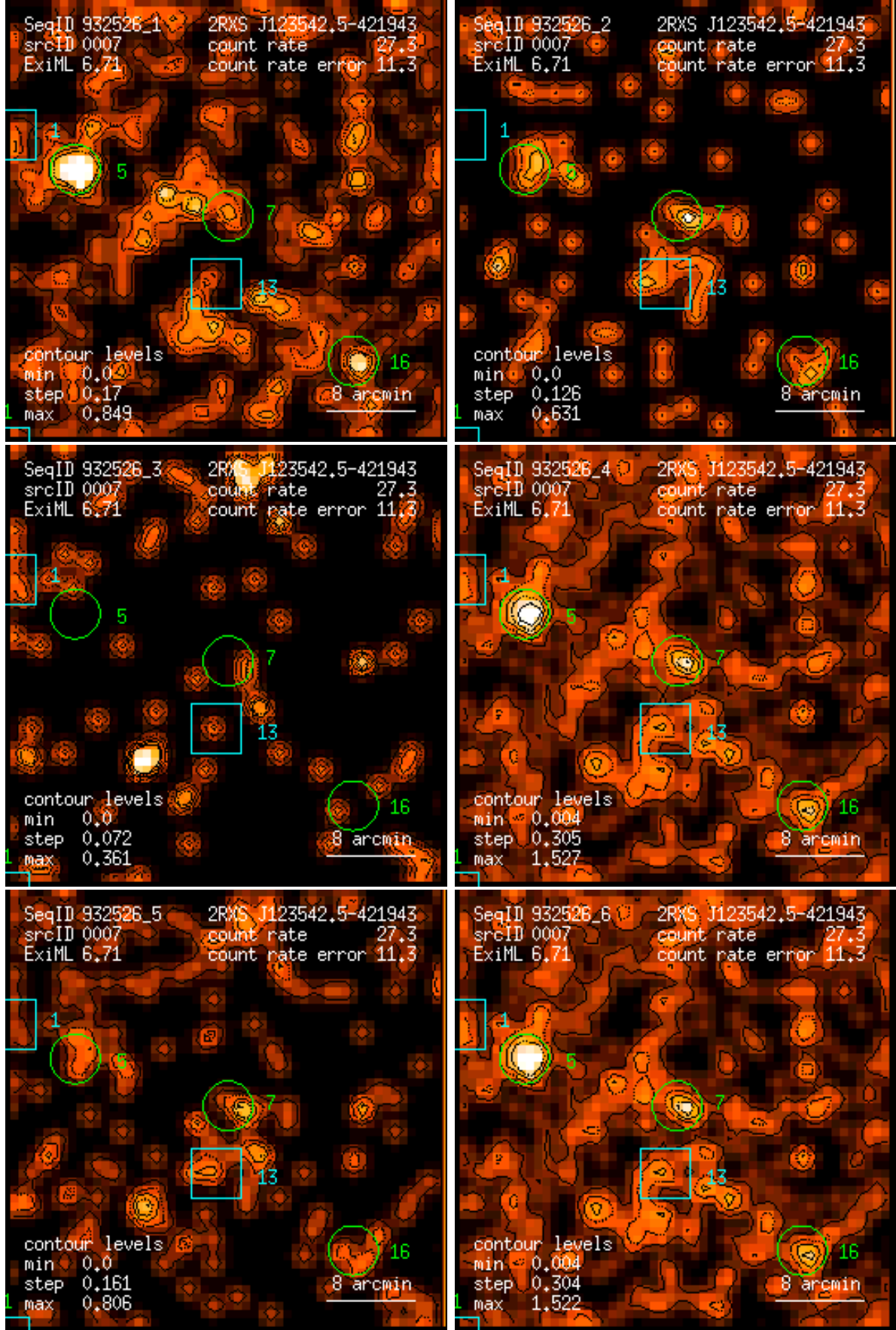
Figure 7: RASS 932526: detection 0007: band rate images, Gaussian filter: (1) PSPC channels 11 – 41, (2) 52 – 90, (3) 91 – 201, (4) 11 – 235, (5) 52 – 201, (6) 11 – 201. Broad band rates in counts/ks. Band rate contour levels in counts/ks/arcmin 2 .
