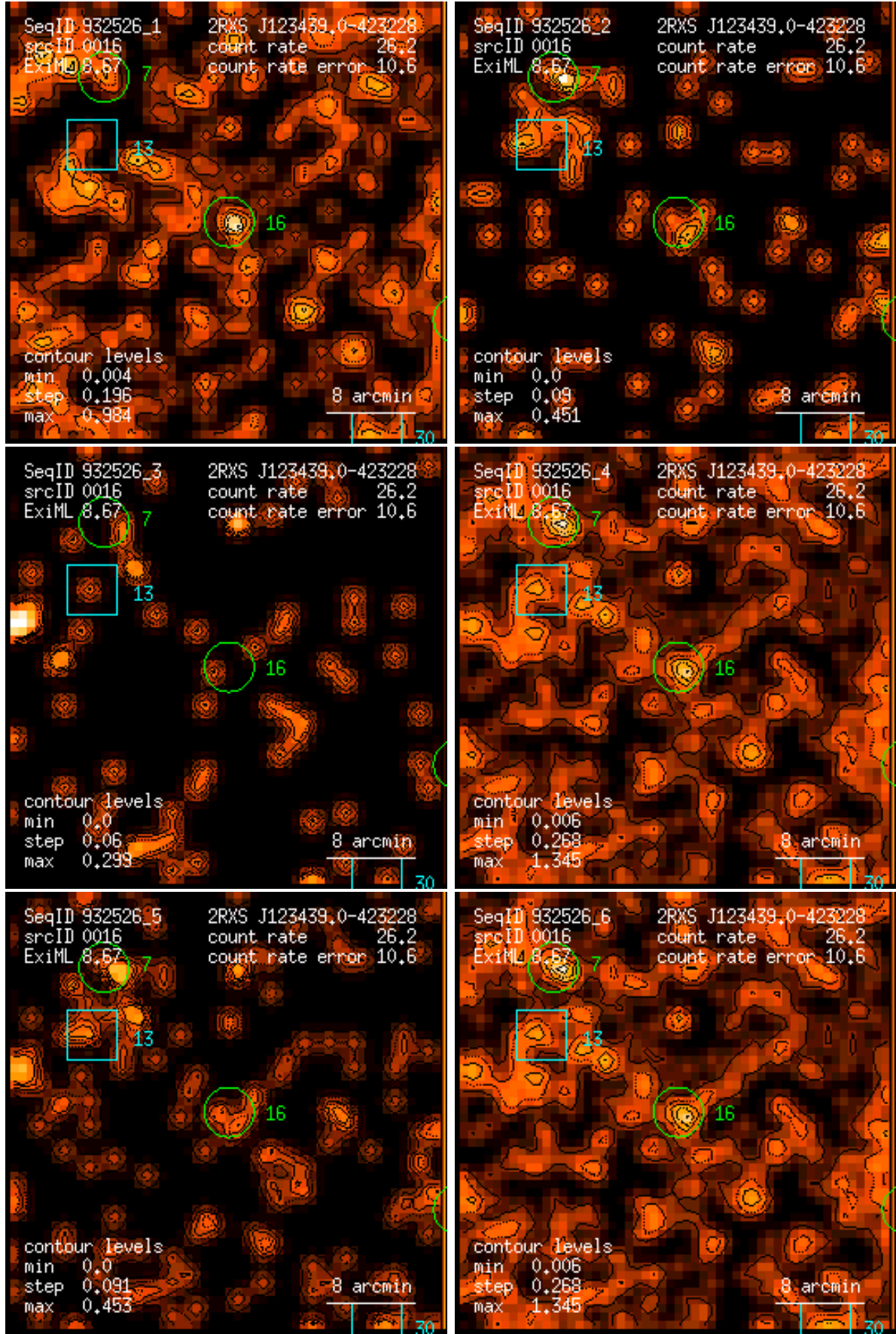
Figure 16: RASS 932526: detection 0016: band rate images, Gaussian filter: (1) PSPC channels 11 – 41, (2) 52 – 90, (3) 91 – 201, (4) 11 – 235, (5) 52 – 201, (6) 11 – 201. Broad band rates in counts/ks. Band rate contour levels in counts/ks/arcmin 2 .
