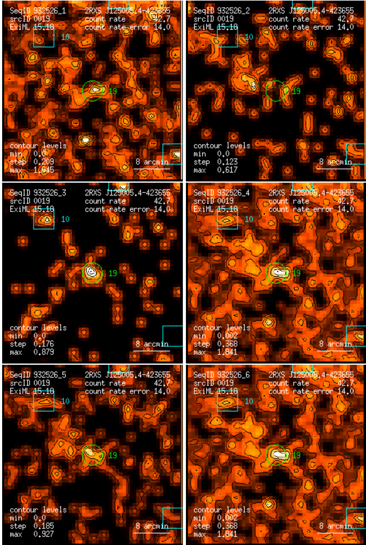
Figure 19: RASS 932526: detection 0019: band rate images, Gaussian filter: (1) PSPC channels 11 – 41, (2) 52 – 90, (3) 91 – 201, (4) 11 – 235, (5) 52 – 201, (6) 11 – 201. Broad band rates in counts/ks. Band rate contour levels in counts/ks/arcmin 2 .
