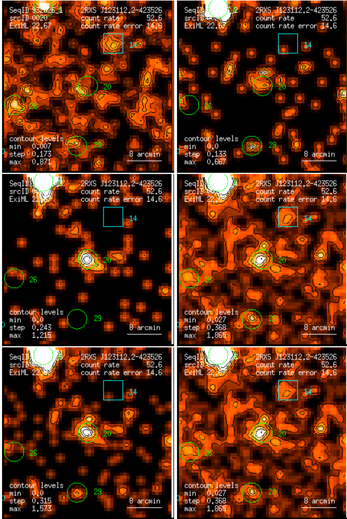
Figure 20: RASS 932526: detection 0020: band rate images, Gaussian filter: (1) PSPC channels 11 – 41, (2) 52 – 90, (3) 91 – 201, (4) 11 – 235, (5) 52 – 201, (6) 11 – 201. Broad band rates in counts/ks. Band rate contour levels in counts/ks/arcmin 2 .
