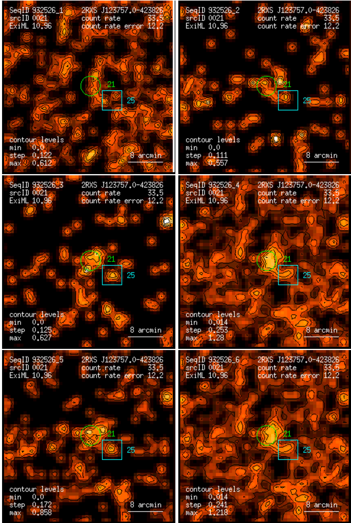
Figure 21: RASS 932526: detection 0021: band rate images, Gaussian filter: (1) PSPC channels 11 – 41, (2) 52 – 90, (3) 91 – 201, (4) 11 – 235, (5) 52 – 201, (6) 11 – 201. Broad band rates in counts/ks. Band rate contour levels in counts/ks/arcmin 2 .
