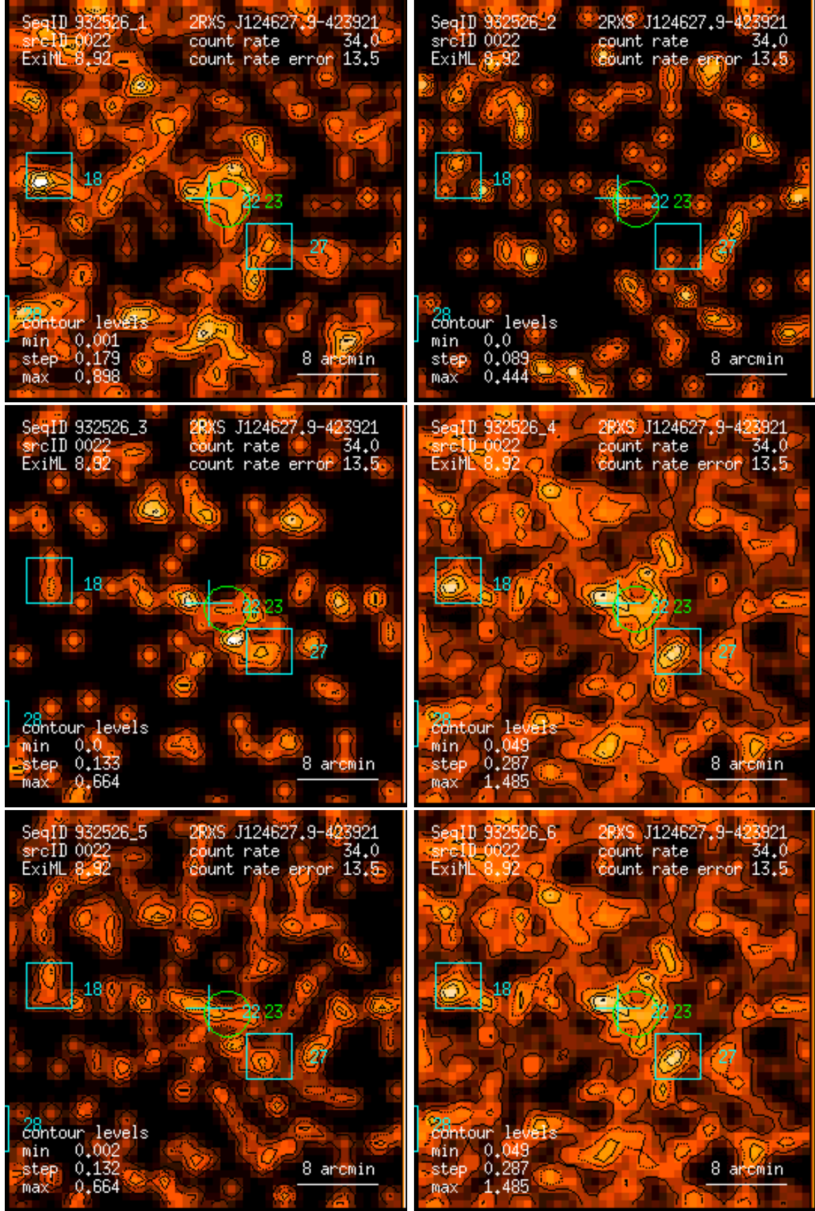
Figure 22: RASS 932526: detection 0022: band rate images, Gaussian filter: (1) PSPC channels 11 – 41, (2) 52 – 90, (3) 91 – 201, (4) 11 – 235, (5) 52 – 201, (6) 11 – 201. Broad band rates in counts/ks. Band rate contour levels in counts/ks/arcmin 2 .
