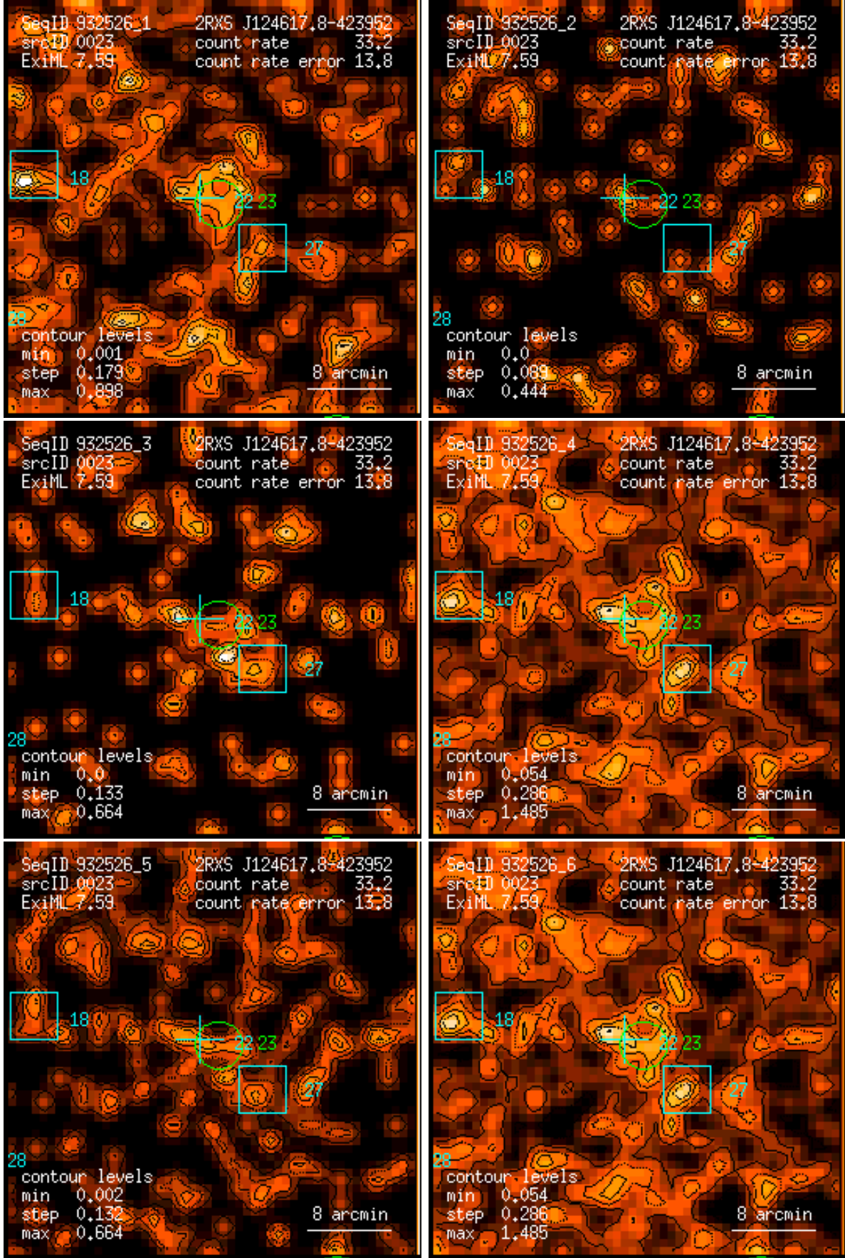
Figure 23: RASS 932526: detection 0023: band rate images, Gaussian filter: (1) PSPC channels 11 – 41, (2) 52 – 90, (3) 91 – 201, (4) 11 – 235, (5) 52 – 201, (6) 11 – 201. Broad band rates in counts/ks. Band rate contour levels in counts/ks/arcmin 2 .
