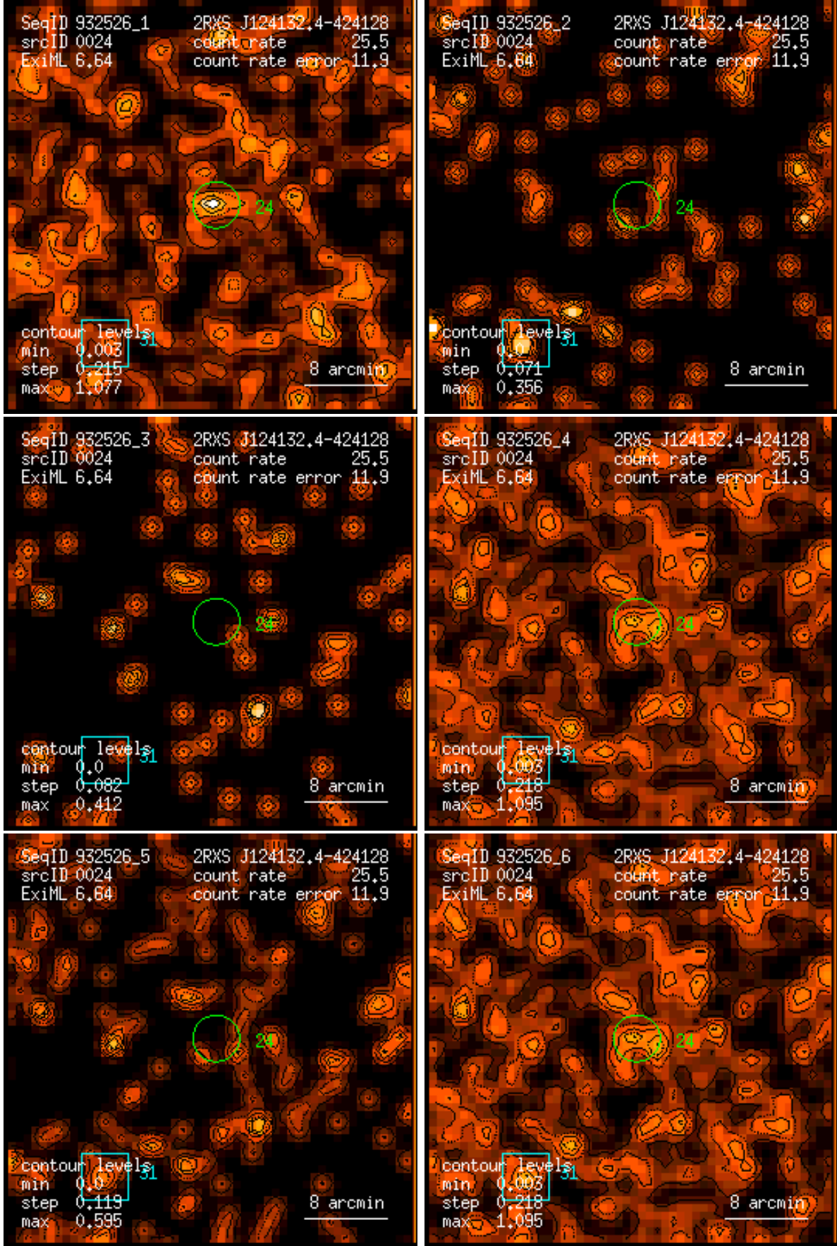
Figure 24: RASS 932526: detection 0024: band rate images, Gaussian filter: (1) PSPC channels 11 – 41, (2) 52 – 90, (3) 91 – 201, (4) 11 – 235, (5) 52 – 201, (6) 11 – 201. Broad band rates in counts/ks. Band rate contour levels in counts/ks/arcmin 2 .
