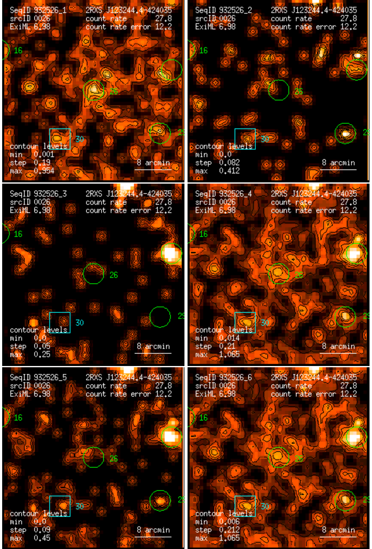
Figure 26: RASS 932526: detection 0026: band rate images, Gaussian filter: (1) PSPC channels 11 – 41, (2) 52 – 90, (3) 91 – 201, (4) 11 – 235, (5) 52 – 201, (6) 11 – 201. Broad band rates in counts/ks. Band rate contour levels in counts/ks/arcmin 2 .
