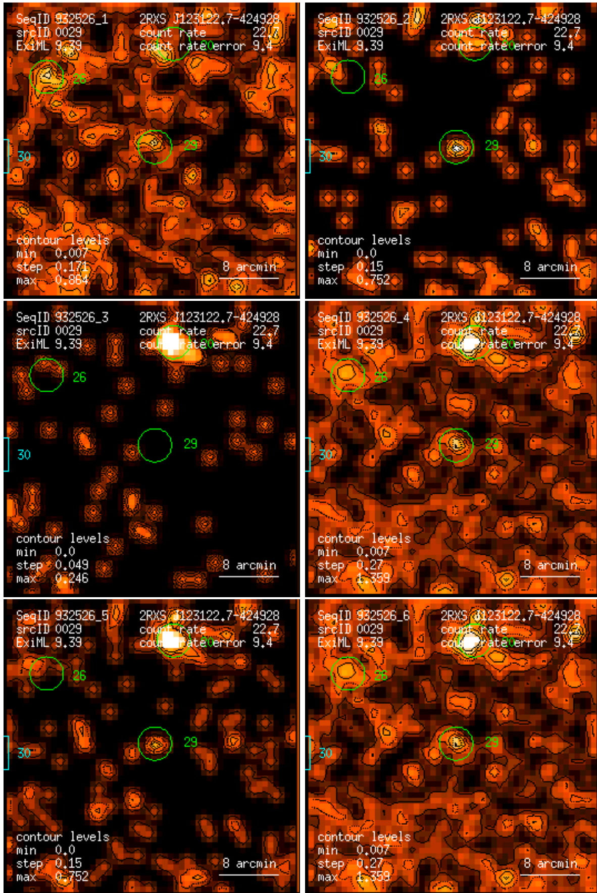
Figure 29: RASS 932526: detection 0029: band rate images, Gaussian filter: (1) PSPC channels 11 – 41, (2) 52 – 90, (3) 91 – 201, (4) 11 – 235, (5) 52 – 201, (6) 11 – 201. Broad band rates in counts/ks. Band rate contour levels in counts/ks/arcmin 2 .
