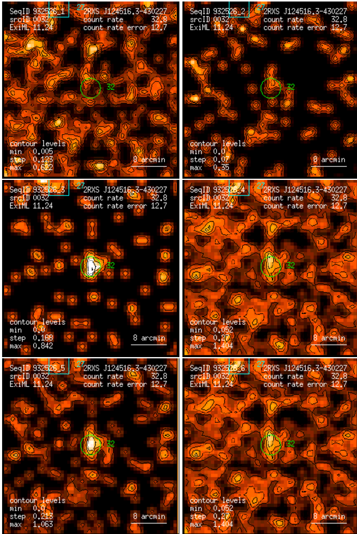
Figure 32: RASS 932526: detection 0032: band rate images, Gaussian filter: (1) PSPC channels 11 – 41, (2) 52 – 90, (3) 91 – 201, (4) 11 – 235, (5) 52 – 201, (6) 11 – 201. Broad band rates in counts/ks. Band rate contour levels in counts/ks/arcmin 2 .
