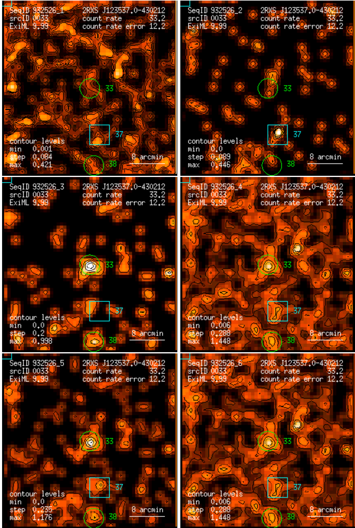
Figure 33: RASS 932526: detection 0033: band rate images, Gaussian filter: (1) PSPC channels 11 – 41, (2) 52 – 90, (3) 91 – 201, (4) 11 – 235, (5) 52 – 201, (6) 11 – 201. Broad band rates in counts/ks. Band rate contour levels in counts/ks/arcmin 2 .
