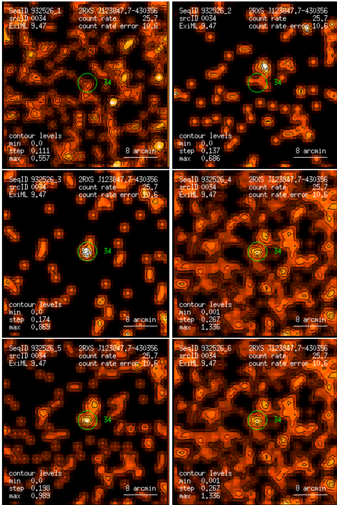
Figure 34: RASS 932526: detection 0034: band rate images, Gaussian filter: (1) PSPC channels 11 – 41, (2) 52 – 90, (3) 91 – 201, (4) 11 – 235, (5) 52 – 201, (6) 11 – 201. Broad band rates in counts/ks. Band rate contour levels in counts/ks/arcmin 2 .
