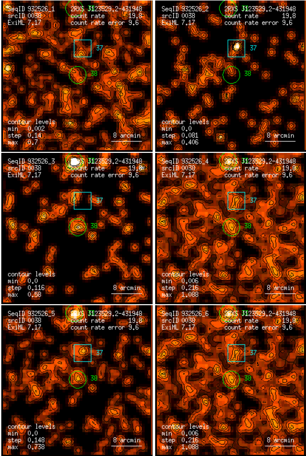
Figure 38: RASS 932526: detection 0038: band rate images, Gaussian filter: (1) PSPC channels 11 – 41, (2) 52 – 90, (3) 91 – 201, (4) 11 – 235, (5) 52 – 201, (6) 11 – 201. Broad band rates in counts/ks. Band rate contour levels in counts/ks/arcmin 2 .
