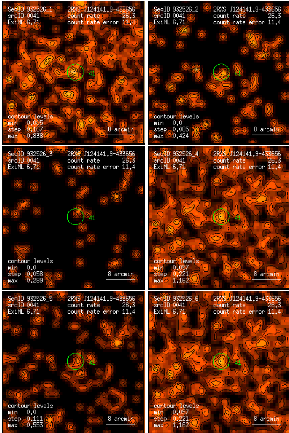
Figure 41: RASS 932526: detection 0041: band rate images, Gaussian filter: (1) PSPC channels 11 – 41, (2) 52 – 90, (3) 91 – 201, (4) 11 – 235, (5) 52 – 201, (6) 11 – 201. Broad band rates in counts/ks. Band rate contour levels in counts/ks/arcmin 2 .
