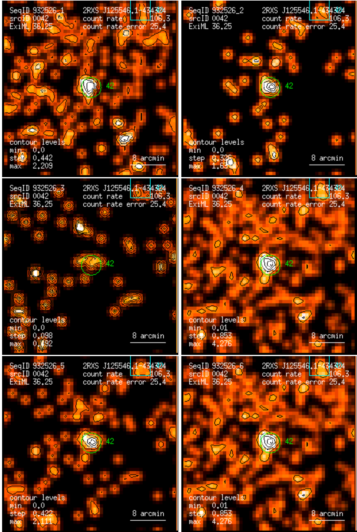
Figure 42: RASS 932526: detection 0042: band rate images, Gaussian filter: (1) PSPC channels 11 – 41, (2) 52 – 90, (3) 91 – 201, (4) 11 – 235, (5) 52 – 201, (6) 11 – 201. Broad band rates in counts/ks. Band rate contour levels in counts/ks/arcmin 2 .
