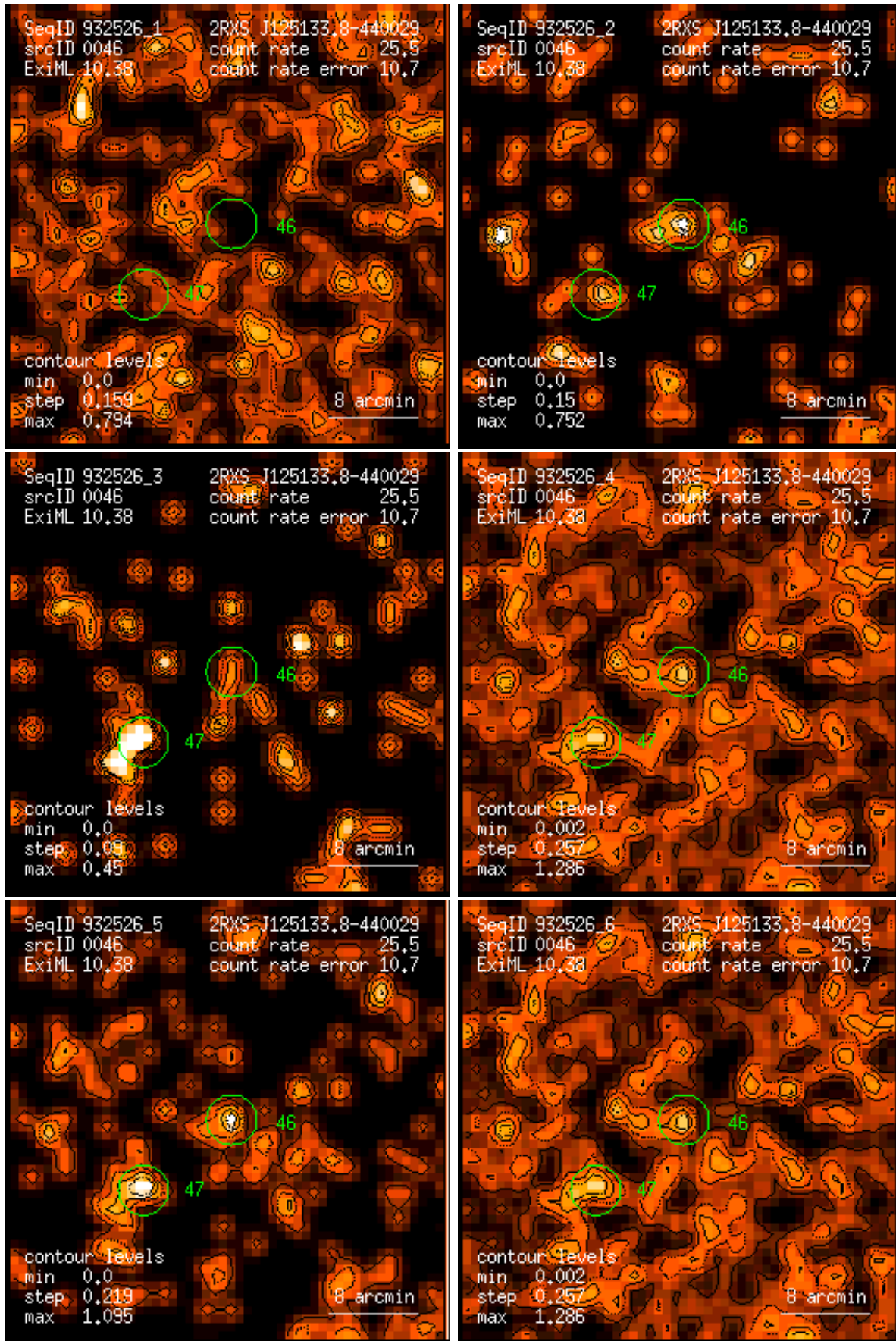
Figure 46: RASS 932526: detection 0046: band rate images, Gaussian filter: (1) PSPC channels 11 – 41, (2) 52 – 90, (3) 91 – 201, (4) 11 – 235, (5) 52 – 201, (6) 11 – 201. Broad band rates in counts/ks. Band rate contour levels in counts/ks/arcmin 2 .
