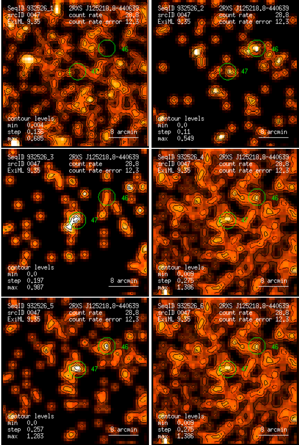
Figure 47: RASS 932526: detection 0047: band rate images, Gaussian filter: (1) PSPC channels 11 – 41, (2) 52 – 90, (3) 91 – 201, (4) 11 – 235, (5) 52 – 201, (6) 11 – 201. Broad band rates in counts/ks. Band rate contour levels in counts/ks/arcmin 2 .
