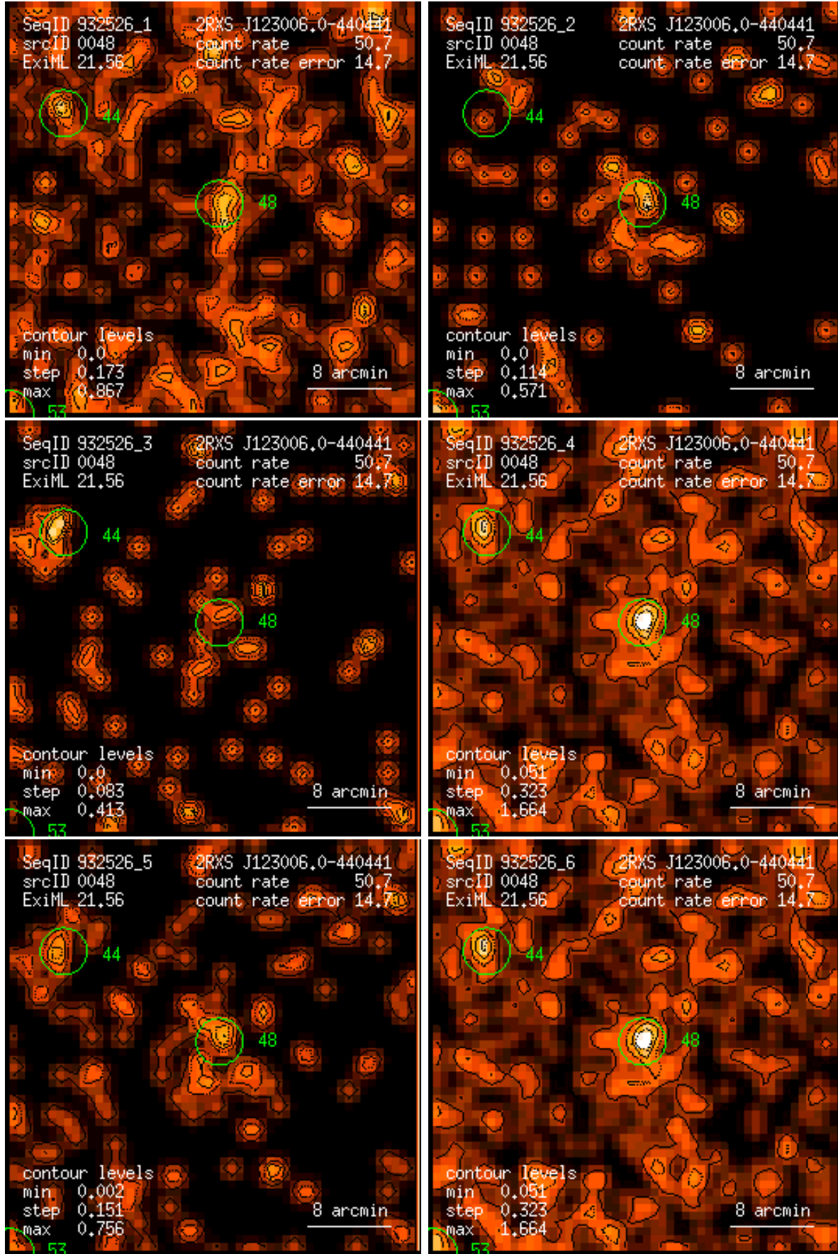
Figure 48: RASS 932526: detection 0048: band rate images, Gaussian filter: (1) PSPC channels 11 – 41, (2) 52 – 90, (3) 91 – 201, (4) 11 – 235, (5) 52 – 201, (6) 11 – 201. Broad band rates in counts/ks. Band rate contour levels in counts/ks/arcmin 2 .
