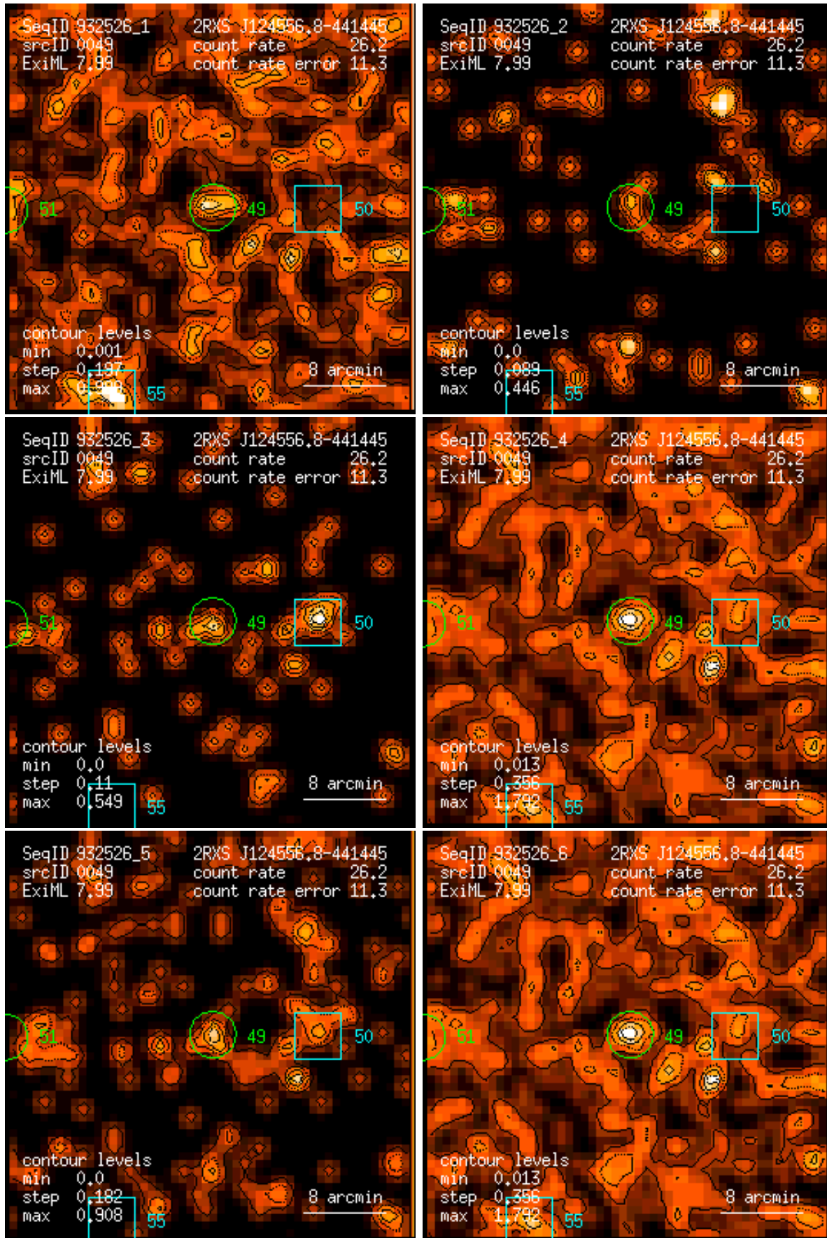
Figure 49: RASS 932526: detection 0049: band rate images, Gaussian filter: (1) PSPC channels 11 – 41, (2) 52 – 90, (3) 91 – 201, (4) 11 – 235, (5) 52 – 201, (6) 11 – 201. Broad band rates in counts/ks. Band rate contour levels in counts/ks/arcmin 2 .
