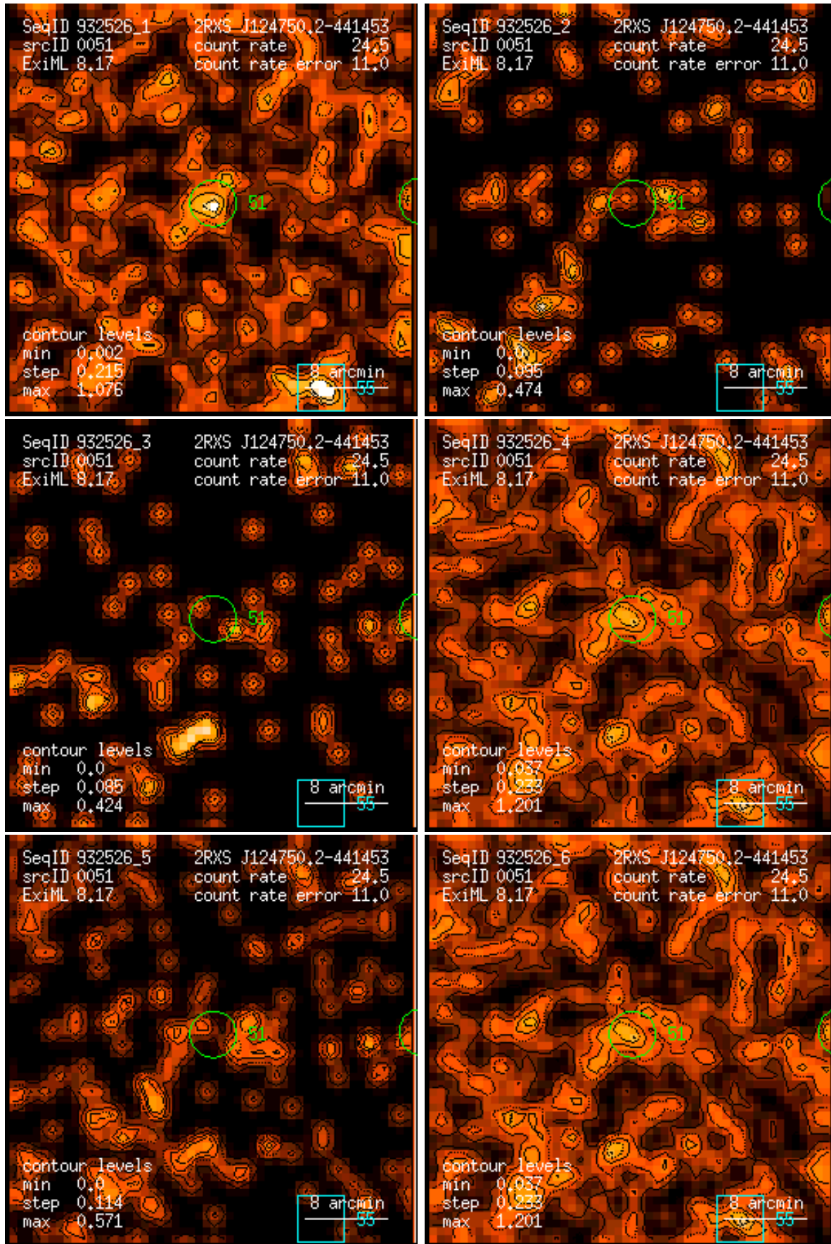
Figure 51: RASS 932526: detection 0051: band rate images, Gaussian filter: (1) PSPC channels 11 – 41, (2) 52 – 90, (3) 91 – 201, (4) 11 – 235, (5) 52 – 201, (6) 11 – 201. Broad band rates in counts/ks. Band rate contour levels in counts/ks/arcmin 2 .
