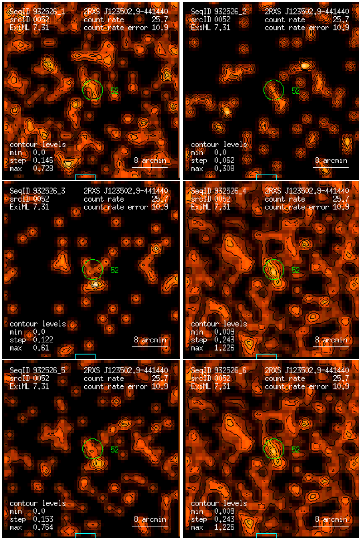
Figure 52: RASS 932526: detection 0052: band rate images, Gaussian filter: (1) PSPC channels 11 – 41, (2) 52 – 90, (3) 91 – 201, (4) 11 – 235, (5) 52 – 201, (6) 11 – 201. Broad band rates in counts/ks. Band rate contour levels in counts/ks/arcmin 2 .
