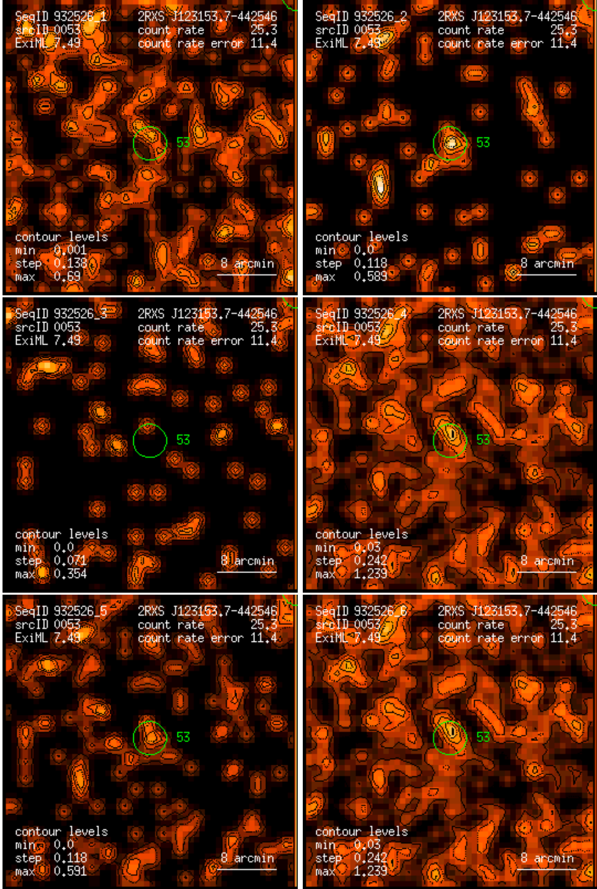
Figure 53: RASS 932526: detection 0053: band rate images, Gaussian filter: (1) PSPC channels 11 – 41, (2) 52 – 90, (3) 91 – 201, (4) 11 – 235, (5) 52 – 201, (6) 11 – 201. Broad band rates in counts/ks. Band rate contour levels in counts/ks/arcmin 2 .
