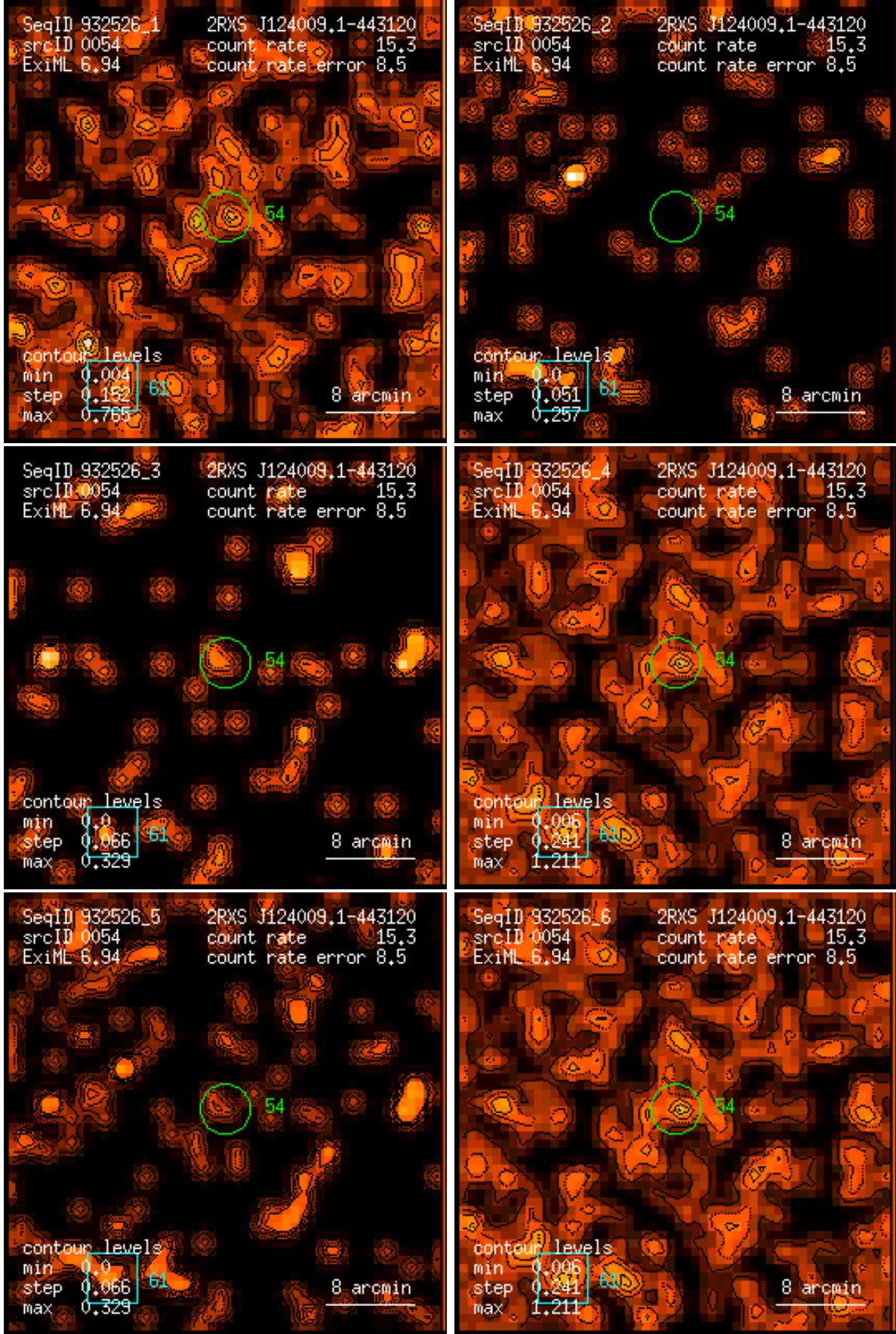
Figure 54: RASS 932526: detection 0054: band rate images, Gaussian filter: (1) PSPC channels 11 – 41, (2) 52 – 90, (3) 91 – 201, (4) 11 – 235, (5) 52 – 201, (6) 11 – 201. Broad band rates in counts/ks. Band rate contour levels in counts/ks/arcmin 2 .
