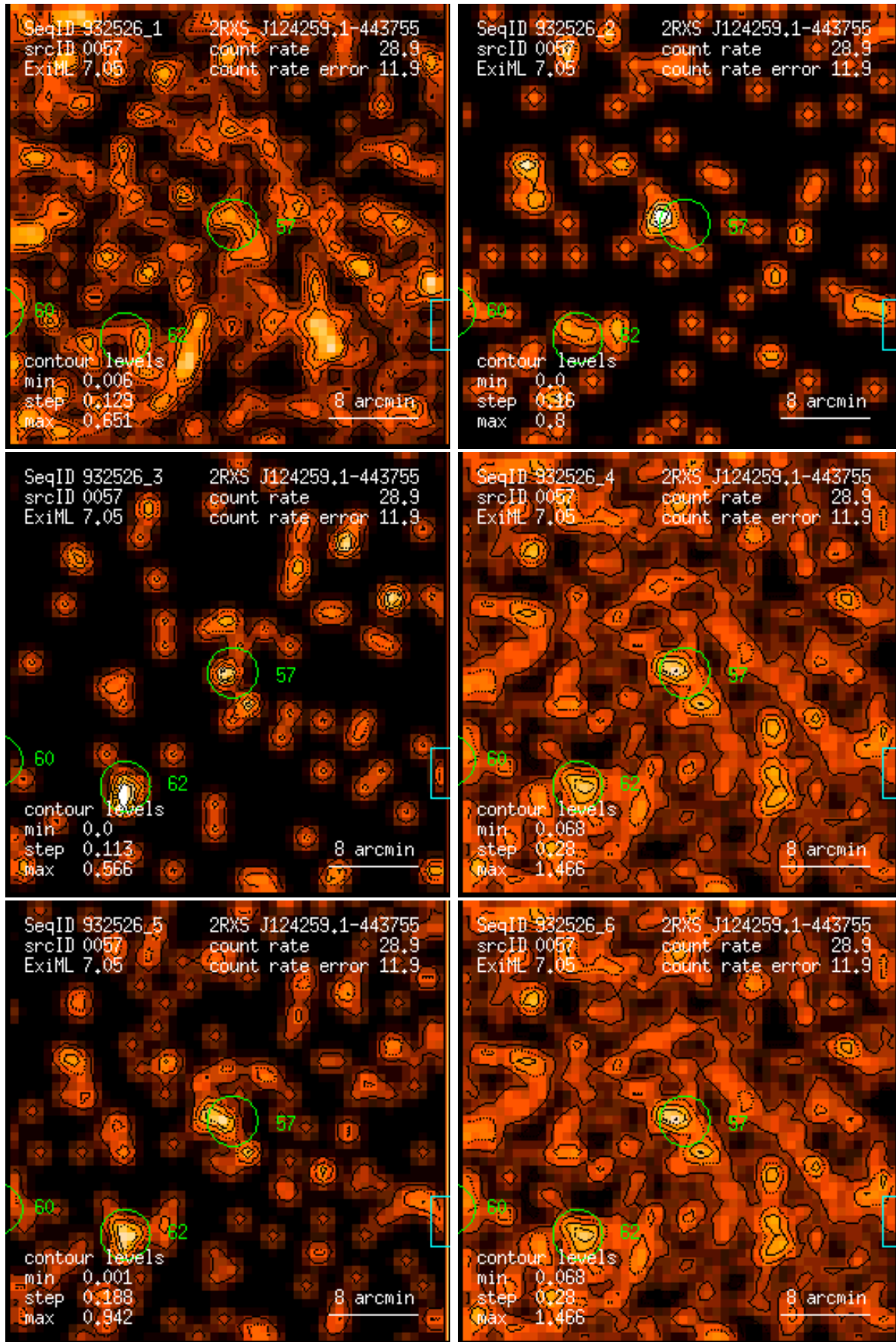
Figure 57: RASS 932526: detection 0057: band rate images, Gaussian filter: (1) PSPC channels 11 – 41, (2) 52 – 90, (3) 91 – 201, (4) 11 – 235, (5) 52 – 201, (6) 11 – 201. Broad band rates in counts/ks. Band rate contour levels in counts/ks/arcmin 2 .
