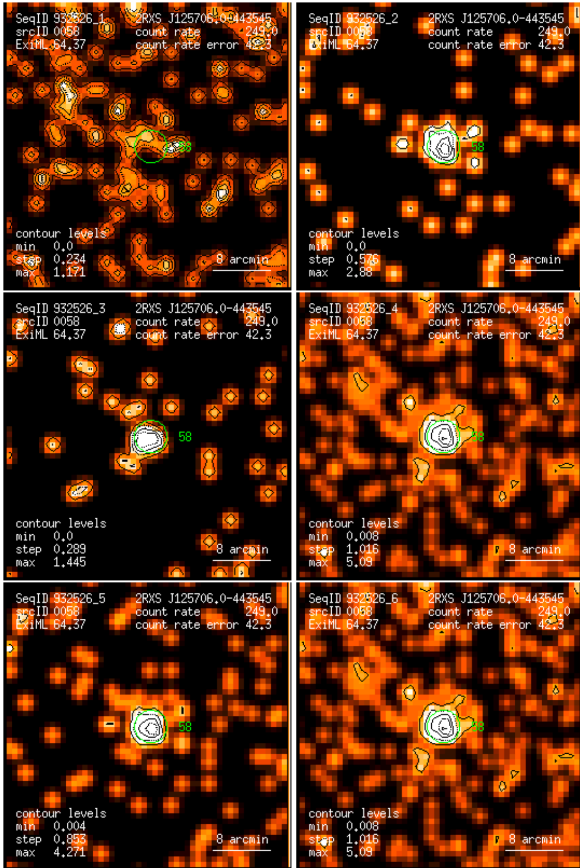
Figure 58: RASS 932526: detection 0058: band rate images, Gaussian filter: (1) PSPC channels 11 – 41, (2) 52 – 90, (3) 91 – 201, (4) 11 – 235, (5) 52 – 201, (6) 11 – 201. Broad band rates in counts/ks. Band rate contour levels in counts/ks/arcmin 2 .
