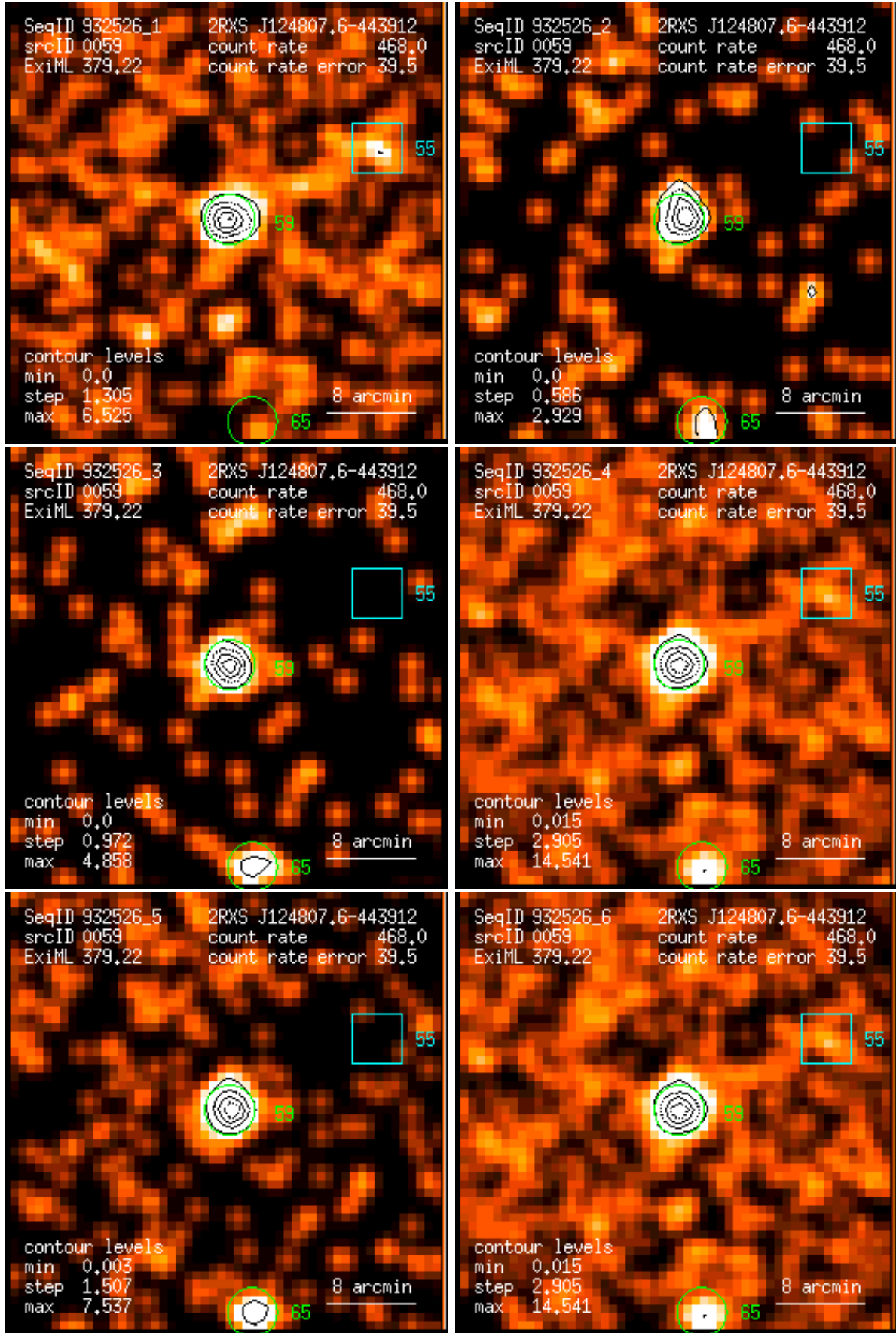
Figure 59: RASS 932526: detection 0059: band rate images, Gaussian filter: (1) PSPC channels 11 – 41, (2) 52 – 90, (3) 91 – 201, (4) 11 – 235, (5) 52 – 201, (6) 11 – 201. Broad band rates in counts/ks. Band rate contour levels in counts/ks/arcmin 2 .
