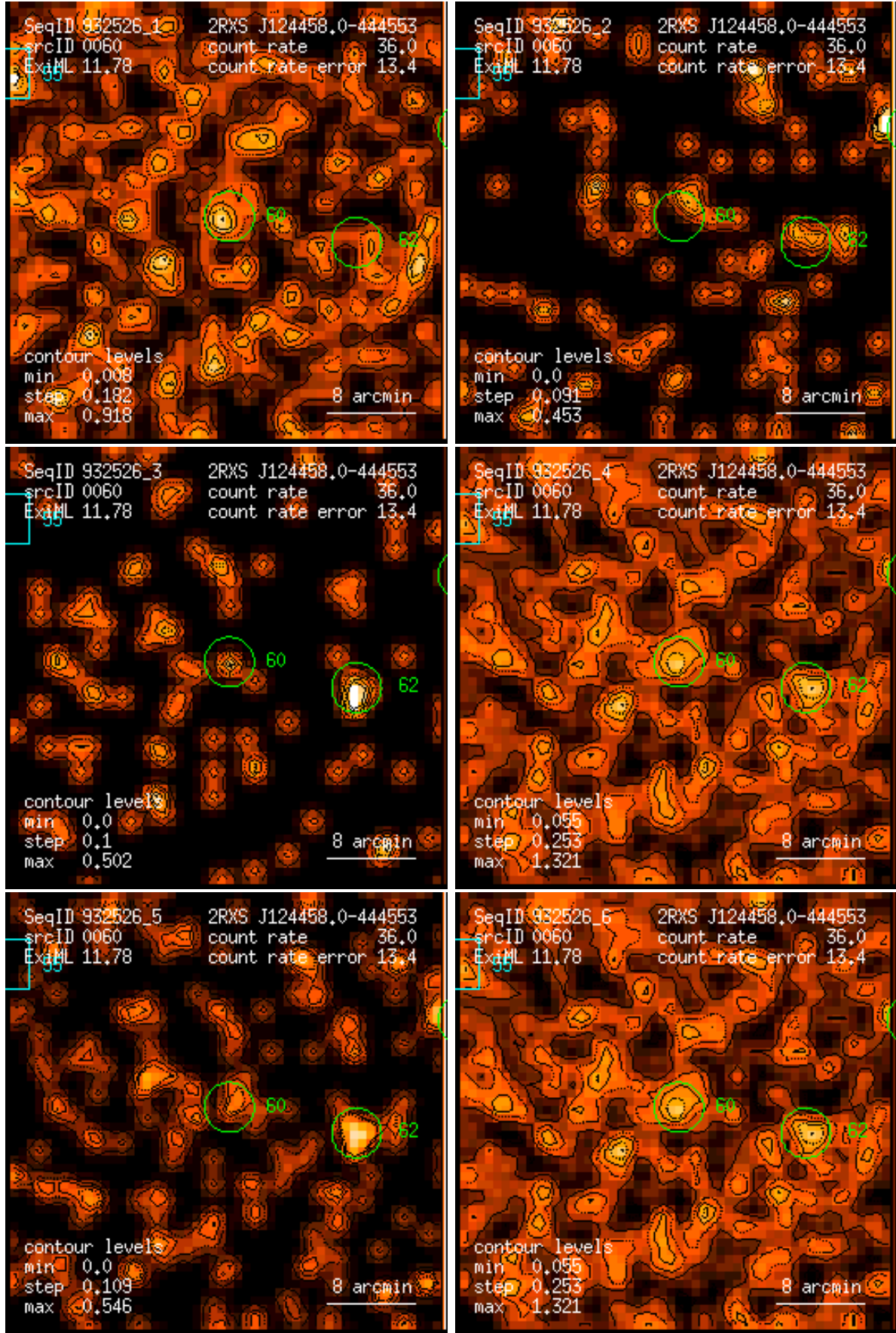
Figure 60: RASS 932526: detection 0060: band rate images, Gaussian filter: (1) PSPC channels 11 – 41, (2) 52 – 90, (3) 91 – 201, (4) 11 – 235, (5) 52 – 201, (6) 11 – 201. Broad band rates in counts/ks. Band rate contour levels in counts/ks/arcmin 2 .
