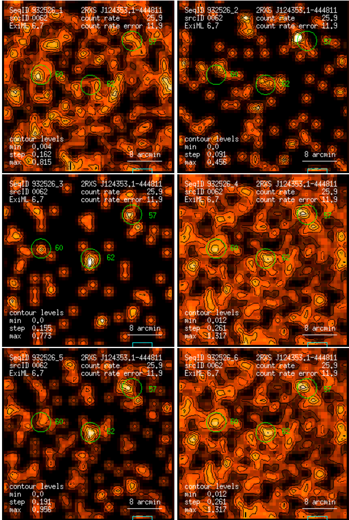
Figure 62: RASS 932526: detection 0062: band rate images, Gaussian filter: (1) PSPC channels 11 – 41, (2) 52 – 90, (3) 91 – 201, (4) 11 – 235, (5) 52 – 201, (6) 11 – 201. Broad band rates in counts/ks. Band rate contour levels in counts/ks/arcmin 2 .
