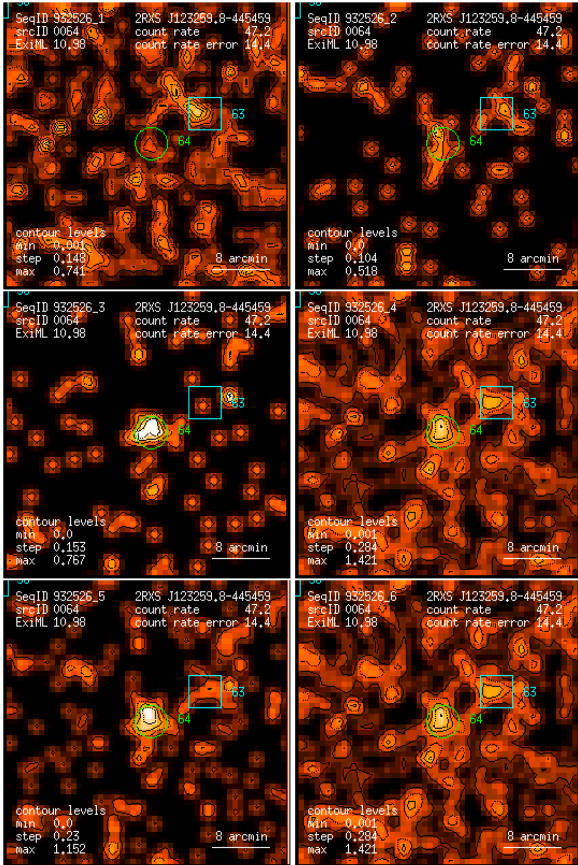
Figure 64: RASS 932526: detection 0064: band rate images, Gaussian filter: (1) PSPC channels 11 – 41, (2) 52 – 90, (3) 91 – 201, (4) 11 – 235, (5) 52 – 201, (6) 11 – 201. Broad band rates in counts/ks. Band rate contour levels in counts/ks/arcmin 2 .
