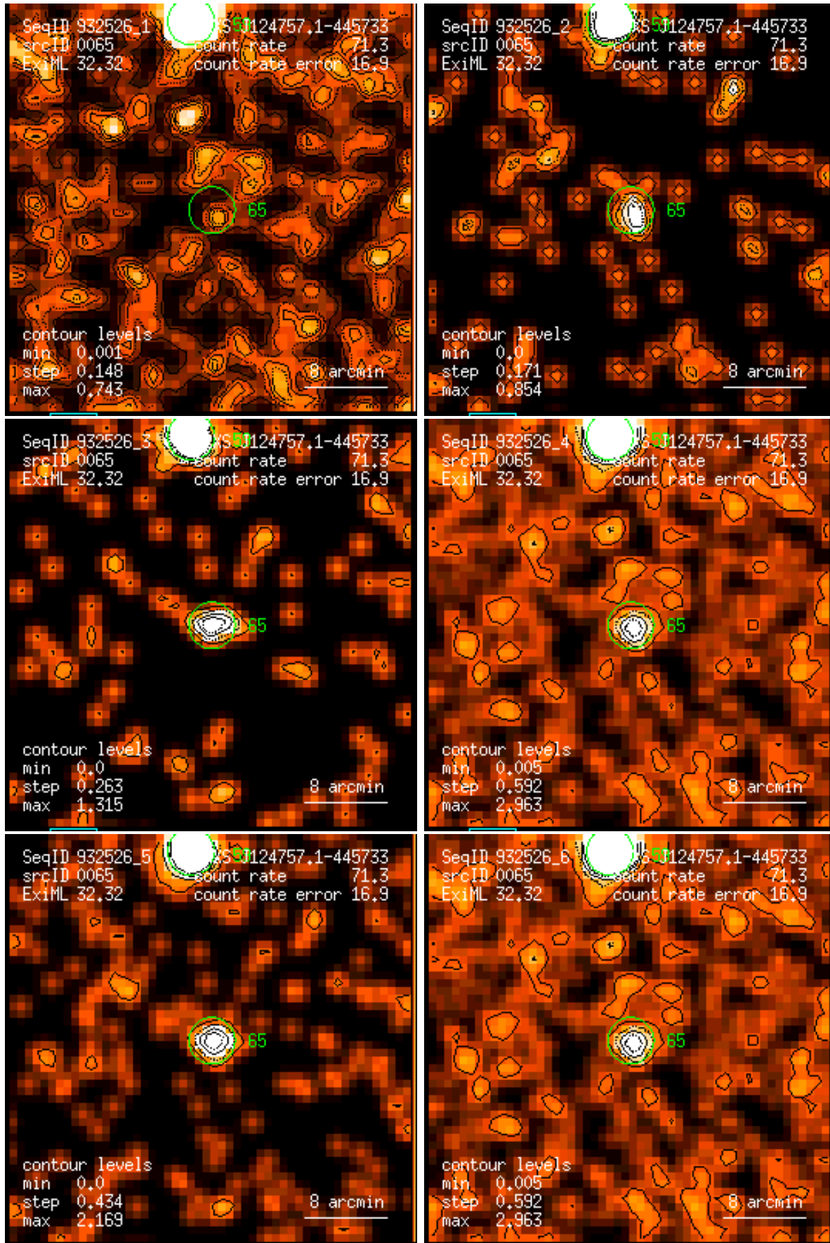
Figure 65: RASS 932526: detection 0065: band rate images, Gaussian filter: (1) PSPC channels 11 – 41, (2) 52 – 90, (3) 91 – 201, (4) 11 – 235, (5) 52 – 201, (6) 11 – 201. Broad band rates in counts/ks. Band rate contour levels in counts/ks/arcmin 2 .
