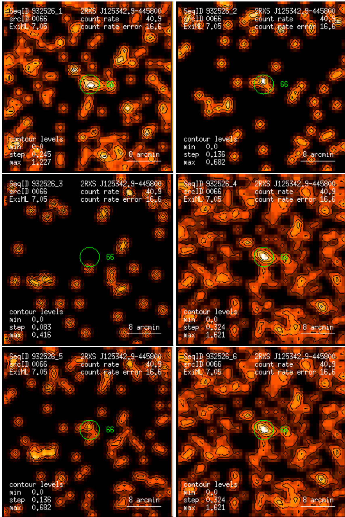
Figure 66: RASS 932526: detection 0066: band rate images, Gaussian filter: (1) PSPC channels 11 – 41, (2) 52 – 90, (3) 91 – 201, (4) 11 – 235, (5) 52 – 201, (6) 11 – 201. Broad band rates in counts/ks. Band rate contour levels in counts/ks/arcmin 2 .
